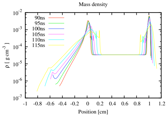
Fig. 4.— Space resolved mass density in the gas cell.
