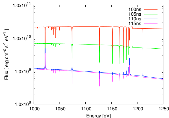
Fig. 5.— Neon K-shell absorption spectra from Spect3d
