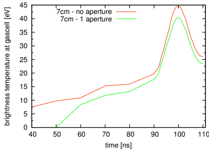
Fig. 1.— Brightness temperature at the gascell front surface with and without aperture in place.
