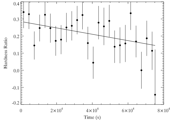
Figure 15. The hardness ratio as a function of time, defined as HR \equiv [CR(>1 \text{ keV}) - CR(<1 \text{ keV})]/[CR(>1 \text{ keV}) + CR(<1 \text{ keV})] , where CR denotes the count rate in the combined zeroth-order and first-order (MEG) data, over the indicated photon energy ranges. We fit a linear function to the data, and find \chi^2 = 25 for 24 degrees of freedom for a constant model (slope of zero), so a constant source model cannot be rejected outright. However, the best-fitting slope of -1.9 \times 10^{-6} \text{ count s}^{-2} (solid line) gives \chi^2 = 20 for 23 degrees of freedom, which is a statistically significant improvement over the constant model.
