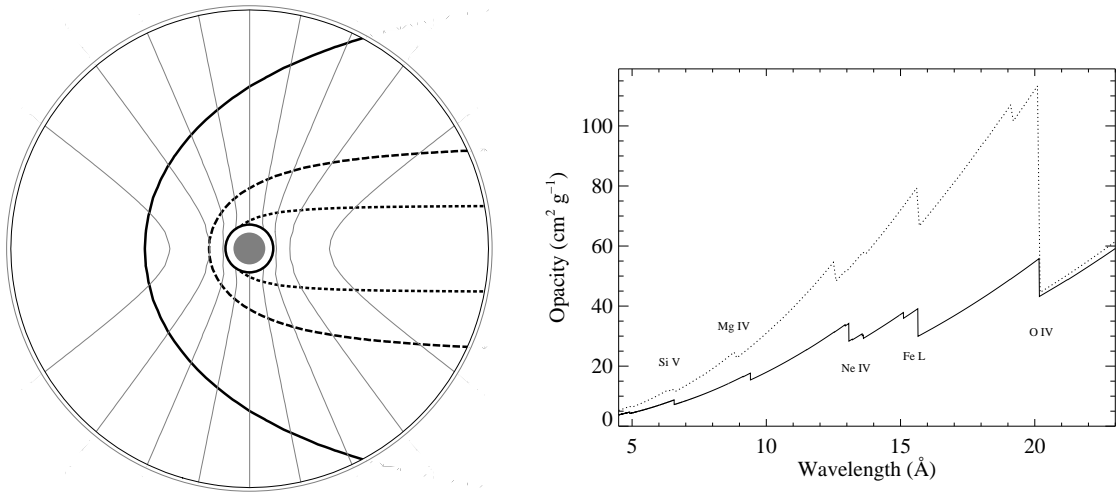
FIGURE 1. In the left panel is a schematic of the scenario that leads to the Doppler broadened and asymmetric x-ray emission line profiles. The observer is on the left, and the dotted lines are contours of constant line-of-sight velocity. These show the Doppler shift of the emitted photons. The gray circle at the center represents the star, and the white annulus around it shows the region below which there is assumed to be no x-ray emission (so that the circle at the outer edge of the annulus represents the adjustable parameter R_o ). The three other lines are contours of constant optical depth ( \tau = 0.3, 1 and 3 for the solid, long dashed, and short dashed contours, respectively). The particular model shown here has R_o = 1.5 R_* and \tau_* = 2 . On the right we show two models for the wavelength-dependent continuum opacity of the bulk, unshocked wind. The dotted line uses a solar abundance mixture of elements, while the solid line represents a model that assumes a particular set of elemental abundances measured from UV and optical spectra of the massive star, \zeta Puppis. The atomic opacity is due to photoelectric absorption, with inner shell absorption edges labeled.
