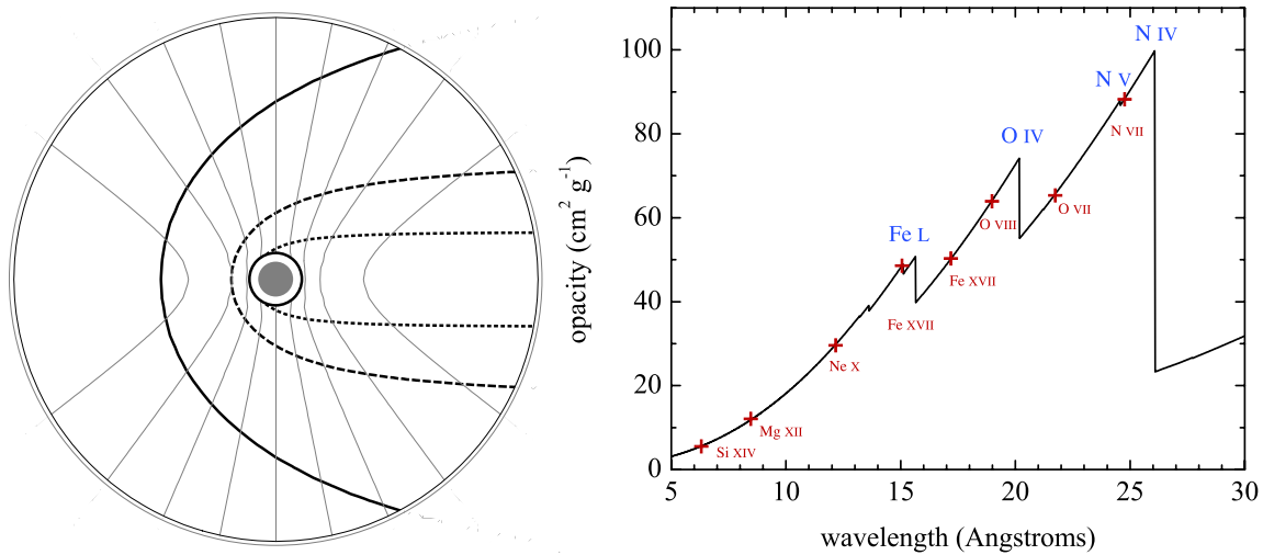
FIGURE 1. In the left panel we show a schematic of the scenario that leads to the Doppler broadened and asymmetric x-ray emission line profiles. The observer is on the left, and the dotted lines are contours of constant line-of-sight velocity. These show the Doppler shift of the emitted photons. The gray circle at the center represents the star, and the white annulus around it shows the region below which there is assumed to be no x-ray emission (so that the circle at the outer edge of the annulus represents the adjustable parameter R_o ). The three other lines are contours of constant optical depth ( \tau = 0.3, 1 and 3 for the solid, long dashed, and short dashed contours, respectively). On the right we show a model for the wavelength-dependent continuum opacity of the bulk, unshocked wind. This model assumes a particular set of abundances (mix of elements) measured from UV and optical spectra of the massive star, \zeta Puppis. The atomic opacity is due to photoelectric absorption, with inner shell absorption edges labeled above the curve in blue. The wavelengths of some important emission lines seen the Chandra emission spectrum of this star are indicated by (red) crosses superimposed on the opacity model (with the parent ions of these lines indicated with labels below the curve).
