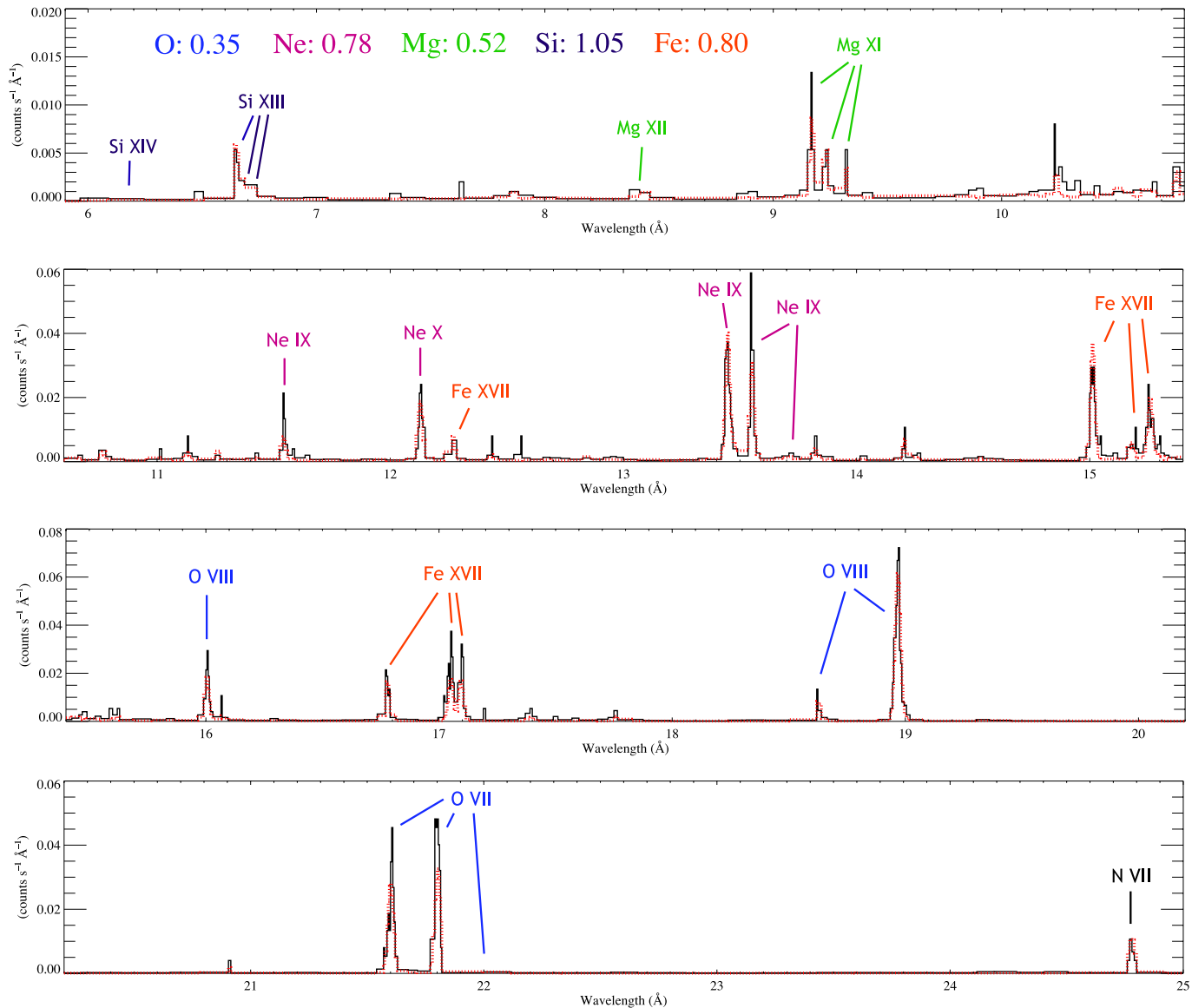
Figure 4. The best-fit two-temperature, variable abundance thermal spectral (vAPEC) model (dotted line; red in on-line color version; parameters listed in Tab. 3; same model as shown in Fig. 3), superimposed on the adaptively smoothed co-added MEG first-order spectrum of \beta Cru. Emission lines are labeled and color coded according to element, with the abundances of each element listed at the top of the figure. Some non-detected lines are labeled, including the forbidden line of O VII near 22.1 Å and the Lyman-alpha line of Si XIV near 6.2 Å.
