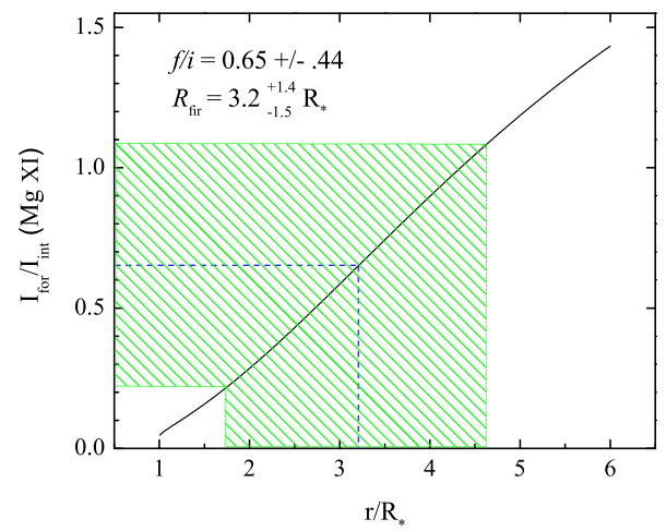
Figure 10. The Mg XI resonance-intercombination-forbidden complex in the co-added MEG data, with the best-fit wind-profile models overplotted (top). The constraints on the formation radius, R_{\text{fir}} , are shown in the bottom panel.
