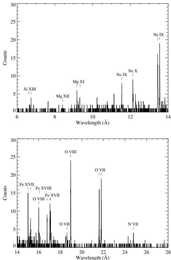
Figure 3. The MEG spectrum of \beta Cru, with negative and positive first orders coadded and emission lines identified by ion. Bins are 5 \text{ m\AA} wide, and each emission line spans several bins. We show a smoothed version of these same data in Fig. 5.
