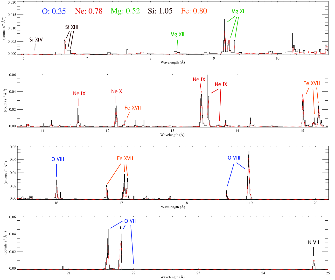
Figure 5. The best-fit two-temperature, variable abundance thermal spectral (APEC) model (dotted line; red in on-line color version; parameters listed in Tab. 3; same model as shown in Fig. 4), superimposed on the adaptively smoothed co-added MEG first-order spectrum of \beta Cru. Emission lines are labeled and color coded according to element, with the abundances of each element listed at the top of the figure. Some non-detected lines are labeled, including the forbidden line of O VII near 22.1 Å and the Lyman-alpha line of Si XIV near 6.2 Å. The N Lyman-alpha line is labeled in black, as we cannot accurately constrain its abundance because only one line is measured.
