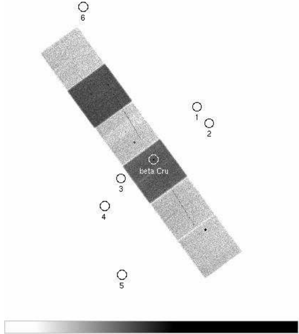
Figure 2. The orientation of the ACIS detector was such that none of the purported PMS stars identified by Park & Finley (1996) (positions shown as dark circles) fall on the chip. Note that the dispersed first order MEG spectrum (-1 and +1 orders) can be seen as two dark bands imaged on the ACIS chips.
