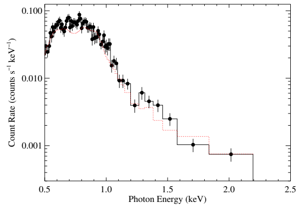
Figure 4. The best-fit two-temperature, variable abundance thermal spectral (APEC) model (dotted line), corrected for pileup, superimposed on the zeroth-order spectrum of \beta Cru. The model shown is the best-fit model fit to both the zeroth and first order spectra, with parameters listed in Tab. 3. It seems likely that some of the systematic deviations in the softer channels are due to optical contamination, as discussed in §4.1.1.
