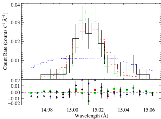
Figure 8. The Fe XVII line at 15.014 Å with three different wind profile models. The dashed line (red in on-line color version) is a constant-velocity wind model with v_\infty = 280 km s ^{-1} (the best-fit value for a constant outflow velocity, which produces emission lines with v_{\text{hwhm}} \approx 150 km s ^{-1} ). The model with v_\infty = 2000 km s ^{-1} , \beta = 1 , and R_{\text{min}} = 1.5 R_* is represented by the dot-dash line (blue in on-line color version). An infinitely narrow model is shown as the dotted line (green in on-line color version). The residuals for each model fit are shown in the lower panel, as red circles for the global best-fit, modestly broadened ( v_\infty = 280 km s ^{-1} ) model, green squares for the narrow profile model, and blue triangles for the broad wind model. The wind model with the higher velocity ( v_\infty = 2000 km s ^{-1} ) clearly does not provide a good fit, while the narrower constant velocity ( v_\infty = 280 km s ^{-1} ) wind model does. And while the very narrow model cannot be absolutely ruled out, the v_\infty = 280 km s ^{-1} model is preferred over it with a high degree of significance. All the models shown here have been convolved with the instrumental response function.
