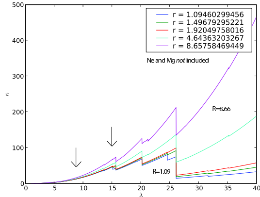
Figure 3: Model of the radius-dependent X-ray opacity as a function of wavelength in the wind of \zeta Pup computed with XCMFGEN. The arrows indicate the wavelengths of the two lines shown in the simulations in Fig. 4.
