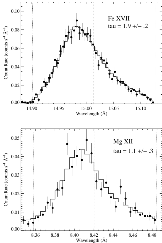
Figure 4: Simulated data for the Fe xvii line at 15.014 Å (top; compare to Fig. 1) and Mg xii Ly-alpha at 8.421 Å (bottom). The simulations assumed a fiducial wind optical depth of \tau_* = 2 for the Fe xvii line and \tau_* = 1 for the Mg xii line (note the larger shift and asymmetry in the higher \tau_* line). When we fit these simulated data with our wind profile model, we derive optical depths of \tau_* = 1.9 \pm 0.2 and \tau_* = 1.1 \pm 0.3 , respectively. Thus the proposed 210 ks exposure will enable us to determine if the wind opacity truly is gray, as would be expected in a porosity-dominated wind. If the expected wavelength dependence is instead seen, as in these simulations, then a significant mass-loss rate reduction would be the favored interpretation.
