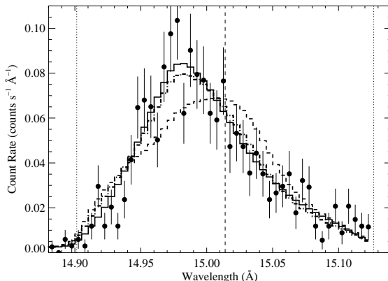
Figure 1: A Fe XVII emission line in the archival Chandra MEG spectrum of \zeta Pup, shown along with three models. The vertical lines represent the line’s rest wavelength and the Doppler shifts associated with the wind terminal velocity. The solid histogram is the best-fit non-porous model, from which we derive a low optical depth, implying a mass-loss rate four times below the literature value. If we allow for porosity, assuming spherical clumps, then we can fit this line with the higher, literature mass-loss rate, but the best-fit model (dash-dot histogram) requires a large interclump spacing of 3.3 R_* (see Fig. 2). The dashed histogram represents the best-fit porous model with flattened (oblate) clumps instead of spherical ones. Here the interclump spacing is even higher, and the fit is statistically ruled out.
