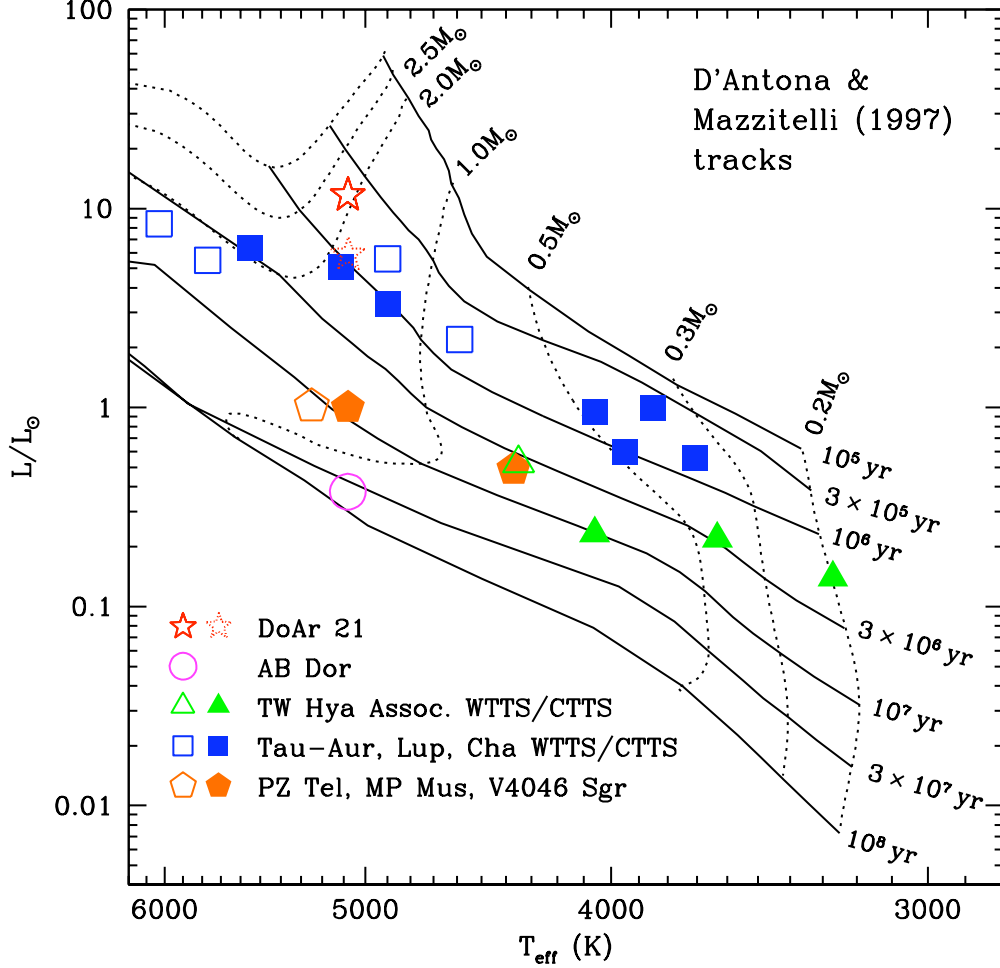
Fig. 1.— HR diagram showing the position of DoAr 21 (star symbols) compared to other pre-main-sequence stars that have been observed with the Chandra or XMM-Newton gratings. The dotted star shows the luminosity of each star in DoAr 21 if it is an equal-mass binary. Filled symbols are classical T Tauri stars, and open symbols are weak-lined T Tauri stars. DoAr 21 is both younger ( \sim 4 \times 10^5 yr) and more massive ( \sim 2.2 M_{\odot} ) than most of the T Tauri stars observed previously. The pre-main-sequence evolutionary tracks shown are from D’Antona & Mazzitelli (1997). Both the Palla & Stahler (1999) and Siess, Dufour, & Forestini (2000) tracks result in slightly older absolute ages in general, but similar relative ages.
