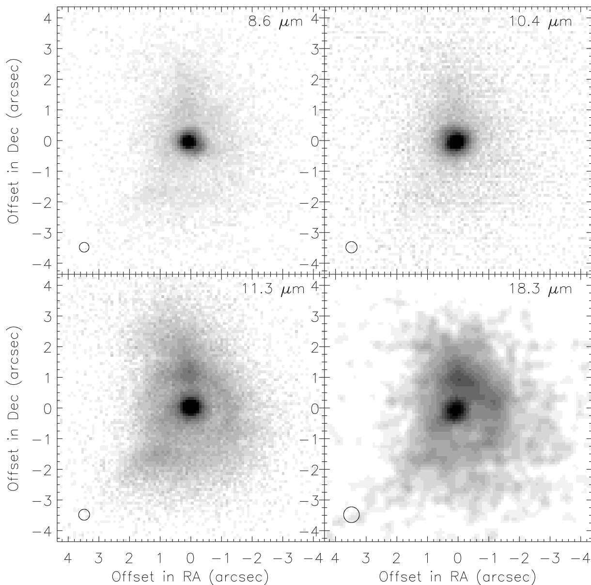
Fig. 4.— Gemini T-ReCS images of DoAr 21 at four different wavelengths. The 8.6- and 11.3- \mu\text{m} bands are centered on PAH emission features, while the other two bands trace continuum emission. The grayscale shows the emission displayed with a logarithmic stretch; the 18.3- \mu\text{m} image is smoothed with a 3-pixel FWHM Gaussian. The circle in the lower left of each image shows the FWHM of the PSF measured from a comparison star observed at similar airmass.
