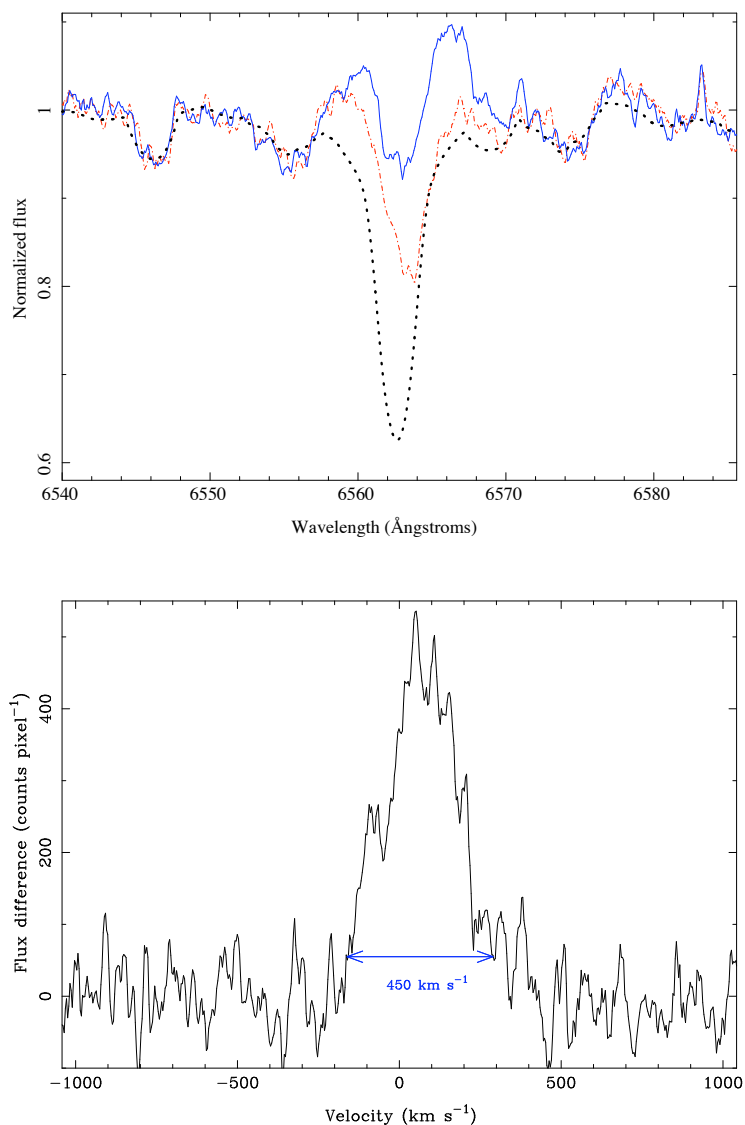
Fig. 7.— High-resolution optical spectra of DoAr 21 in the vicinity of the H\alpha line. Top: The dot-dashed line (red in the online edition) shows DoAr 21 on 12 April 2003; the solid line (blue in the online edition) shows DoAr 21 on 13 April 2003; the dotted line shows the K1 V standard star HD 13445, artificially broadened to v \sin i = 80 \text{ km s}^{-1} . The H\alpha line in DoAr 21 clearly is filled in by a broad emission component that is present on both nights, but stronger on the second night. Bottom: The difference between the two DoAr 21 spectra, showing the broad emission component that appears the second night. The full-width at 10% intensity is indicated.
