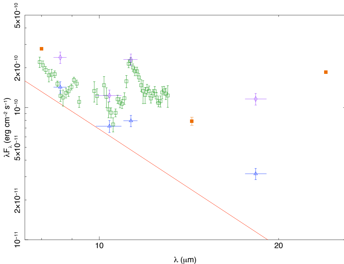
Fig. 6.— A close-up of the mid-infrared SED, with the model photosphere and de-reddened photometry as in Figure 2. The broad-band Spitzer and ISO data are shown as filled squares (orange in the on-line edition), and the spectrum from Hanner et al. (1995) is shown as open squares (green in the on-line edition), showing an emission feature at 11.3 \mu\text{m} attributed to PAHs. De-reddened photometric measurements from new Gemini narrow-band images are overplotted, with horizontal bars showing the bandwidth of the filters used and vertical error bars showing the assumed 10% uncertainty. The open triangles (blue in the on-line edition) show measurements within 100 AU ( 0''.82 ) of the star, showing little or no excess in the continuum at 10.4 \mu\text{m} . The open diamonds (purple in the on-line edition) show measurements in a 2''.75 radius aperture, the same as that used by Hanner et al. (1995).
