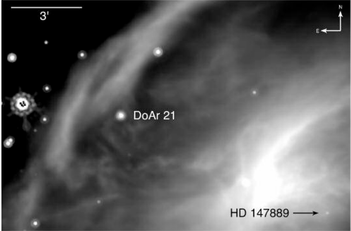
Fig. 3.— Spitzer MIPS 24- \mu m image of the field around DoAr 21; DoAr 21 is clearly detected, indicating a substantial amount of circumstellar material. Unlike other stellar sources in the field, DoAr 21 does not show the first Airy ring, indicating that the 24- \mu m emission is marginally resolved. The B2 star HD 147889 (lower right) excites the emission from the bright ridge to the northeast of DoAr 21.
