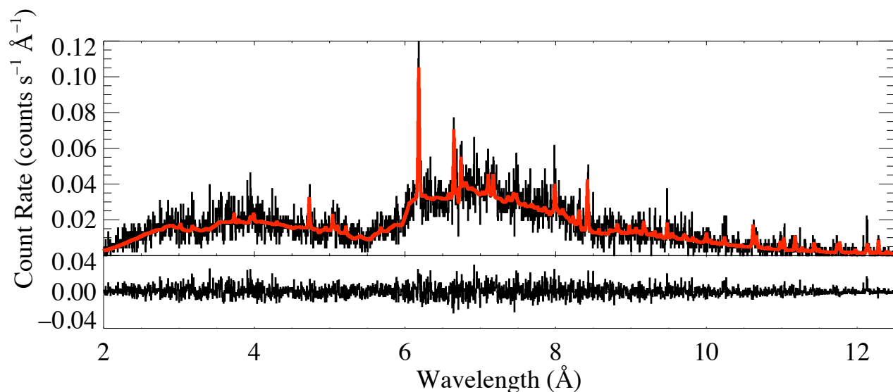
Fig. 9.— The best-fit two-temperature thermal emission model is superimposed (in gray; red in the on-line edition) on the MEG data, with fit residuals shown below.
