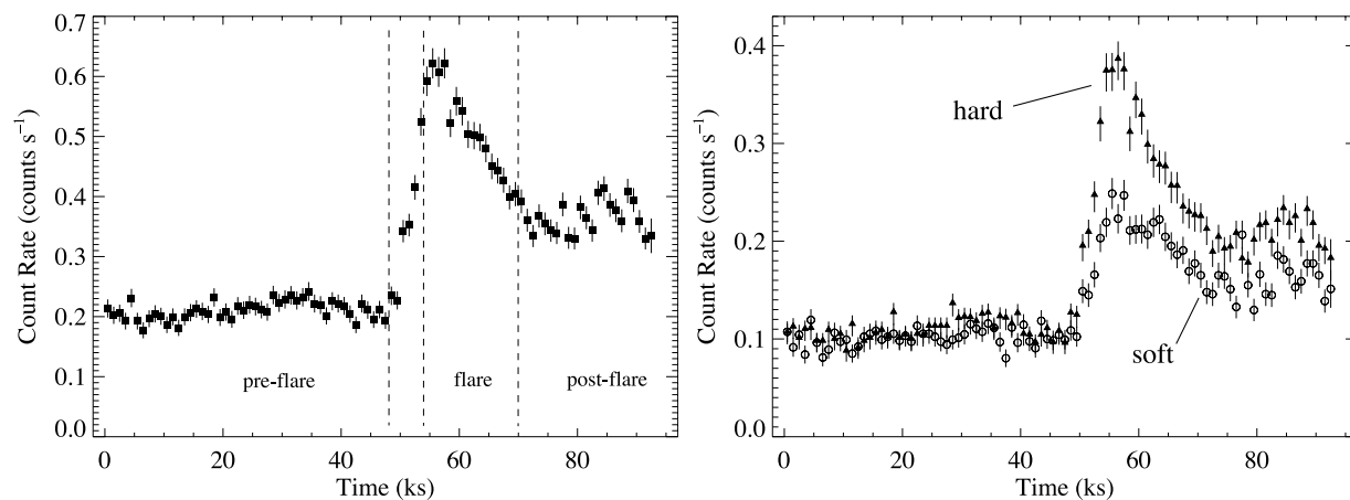
Fig. 10.— Left: A light curve with 1000-second bins formed from all counts in the dispersed, first-order spectra (both MEG and HEG). Right: Light curves made from all counts with wavelengths longer than 6.8 \text{ \AA} (open circles) and shorter than 6.8 \text{ \AA} (filled triangles). The hardening of the emission during and after the flare is evident.
