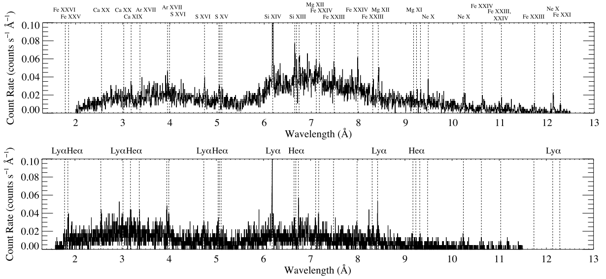
Fig. 8.— The entire usable portions of the MEG (top) and HEG (bottom) co-added (negative and positive) first order spectra of DoAr 21. The bin sizes are 2.5 mÅ for the HEG and 5 mÅ for the MEG. The shape of the continuum is dominated by the wavelength-dependent effective area of the telescope, gratings, and detector, and by interstellar absorption, rather than by the intrinsic emission. Vertical dashed lines represent the laboratory rest wavelengths of all detected emission lines. The annotations above the top panel indicate the element and ionization stage of each line, while those above the lower panel highlight the Lyman- \alpha lines of the hydrogen-like isoelectronic sequence and the principal transition of the helium-like isoelectronic sequence.
