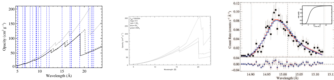
Figure 3. Opacity models that demonstrate the greatest possible radial variation within a single, solar abundance, O star wind are shown in the left panel. Wavelengths of lines measured with the Chandra gratings are indicated by the vertical dashed (blue) lines, while the three different opacity models assume high ionization (metals in +4 and He fully ionized; solid), medium ionization (metals in +3 and He fully ionized; dashed) and low ionization (metals in +2 and He fully recombined to He II; dotted). Clearly, the metal ionization differences are a small effect, and the He recombination is the dominant effect, but is significant only longward of the oxygen K-shell edge near 20 Å. In the middle panel we show opacities specific to ζ Pup, computed via detailed wind modeling using CMFGEN, at three different radii in the wind ( Note: awaiting updated calculation/figure from Janos. ). As expected, the opacity variation is small below the O K-shell edge, and larger above it, although not as large as the maximal scenario presented in the first panel. On the right is a profile fit to the Fe XVII line at 15.014 Å (blue histogram) from a model where the wind opacity triples beyond r \sim 5 R_* (as given by the radial profile in the inset), compared to a model with constant opacity (red histogram). The fit with the outer-wind opacity increase demonstrates a high degree of degeneracy with constant opacity models, but even in this extreme case, the decrease in \tau_* is only 30 per cent, as listed in Table 2.
