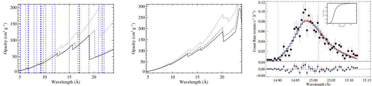
Figure 3. Opacity models that demonstrate the greatest possible radial variation within a single, solar abundance, O star wind are shown in the left panel. Wavelengths of lines measured with the Chandra gratings are indicated by the vertical dashed (blue) lines, while the three different opacity models assume high ionization (metals in +4 and He fully ionized; solid), medium ionization (metals in +3 and He fully ionized; dashed) and low ionization (metals in +2 and He fully recombined to He II; dotted). Clearly, the metal ionization differences are a small effect, and the He recombination is the dominant effect, but is significant only longward of the oxygen K-shell edge near 20 Å. In the middle panel we show opacities specific to \zeta Pup, computed via detailed wind modeling using CMFGEN, at three different radii in the wind (1.4, 3.9, 9.6 R_* from solid to dashed, to dotted). (Note that the overall opacity, especially at long wavelengths, is somewhat higher than solar abundance models because of the helium abundance enhancement in \zeta Pup, and slightly higher than solar metallicity in the CMFGEN model.) As expected, the opacity variation is small below the O K-shell edge, and larger above it, although not as large as the maximal scenario presented in the first panel. On the right is a profile fit to the Fe XVII line at 15.014 Å (blue histogram) from a model where the wind opacity triples beyond r \sim 5 R_* (as given by the radial profile in the inset), compared to a model with constant opacity (red histogram). The fit with the outer-wind opacity increase demonstrates a high degree of degeneracy with constant opacity models, but even in this extreme case, the decrease in \tau_* is only 30 per cent, as can be seen by comparing the first and last rows of Table 2.
