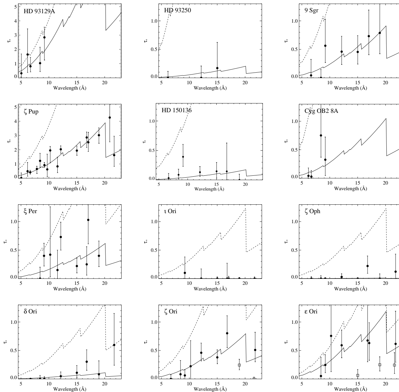
Figure 4. The fitted \tau_* values (points), along with the 68 per cent confidence limits (error bars). The mass-loss rates derived from these values are shown graphically as the solid line, while the dashed line in each panel represents the \tau_* trend expected from the theoretical mass-loss rates listed in Table 3. For \zeta Ori and \epsilon Ori we show the two and three points, respectively, omitted from the mass-loss rate fits because of resonance scattering (open squares). Note that in both stars, the He-like resonance line (at 21.602 Å) has a smaller \tau_* value than the intercombination line (at 21.804 Å), which is indicative of resonance scattering being important.
