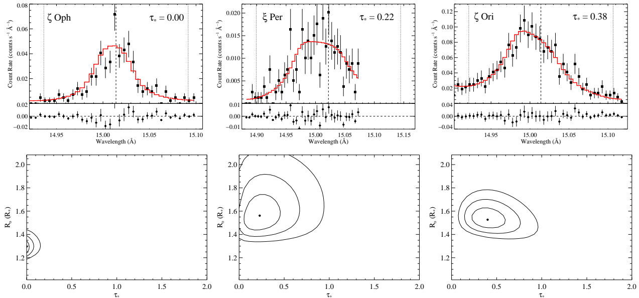
Figure 1. The Fe xvii line at 15.014 \text{\AA} with best-fit model (top row) for three of the sample stars ( \zeta Oph, \tau_* = 0.00^{+.01}_{-.00} (left), \xi Per, \tau_* = 0.22^{+.14}_{-.12} (middle), and \zeta Ori, \tau_* = 0.38^{+.13}_{-.11} (right)) showing various degrees of asymmetry. The vertical dashed lines on the profile plots represent the laboratory line rest wavelength and the wavelengths corresponding to the terminal velocity of the wind. Note that the x-axis in each figure in the top row encompasses the same velocity range in units of the wind terminal velocity, but different absolute velocity and wavelength ranges, due to the different terminal velocities of the three stars' winds. The emission line in \zeta Oph, with the lowest wind terminal velocity, is therefore even narrower, in an absolute sense, than it appears here. And the star with the highest wind velocity, \xi Per, is subject to more blending on its red wing than are the other two stars. The contours in the lower panels give the 68 per cent, 95 per cent, and 99.7 per cent two-dimensional joint confidence limits on \tau_* and R_o , while the best-fit models are indicated by the filled circles.
