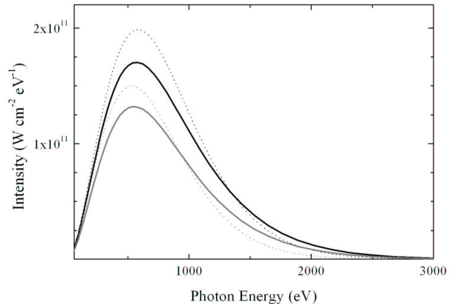
FIG. 3: The simulated DANTE spectrum (solid black) along with the equivalent blackbody spectrum (dotted black) for t = 1.0 ns in the VISRAD hohlraum simulation and the simulated spectrum incident on the hohlraum wall at the midplane (solid gray) along with its equivalent blackbody spectrum (dotted gray) from the same simulation time. Note that the radiation temperatures are 202 eV for DANTE and 188 eV for the midplane wall.
