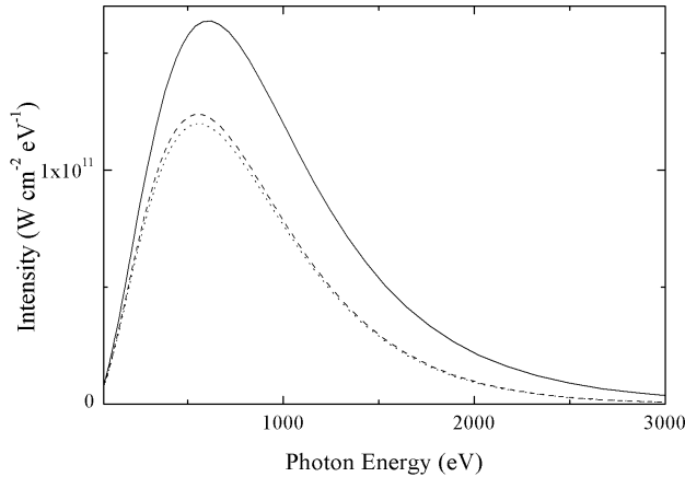
FIG. 19: Comparison of spectra incident on the center of the sample in our standard ( l = 1150 \mu\text{m} ) halfraum at t = 1.0 \text{ ns} , with the standard beam pointing. The dotted line represents the simulation with no foil, the dashed line (nearly coincident with the dotted line) represents the simulation with a foil outside the LEH, and the solid line is from the simulation with the foil heated by ten beams.
