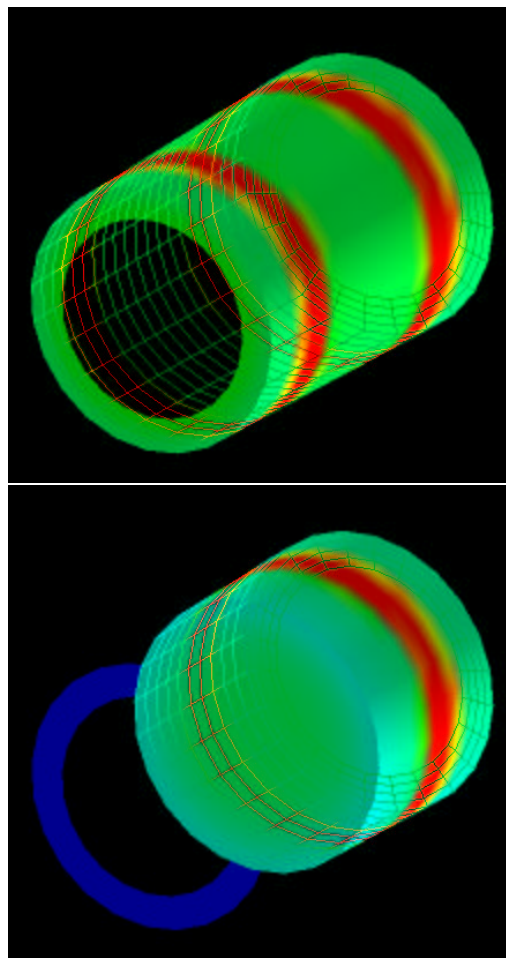
FIG. 7: The DANTE view at t = 1.0 \text{ ns} of our original hohlraum simulation (top) and the same view of a simulation that differs only in having a gold disk dividing the hohlraum in half, effectively turning it into a halfraum (bottom). The temperature color scales are identical in the two figures. Note that from this viewing angle, some of the laser hot spots on the far side of the hohlraum, caused by beams entering the hohlraum through the far LEH, are visible, which is, of course, not the case with the dividing disk present.
