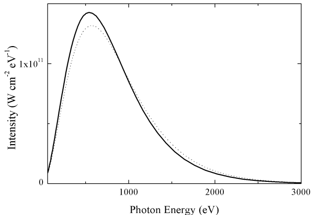
FIG. 6: Comparison of the spectrum incident on a sample at the center of a hohlraum when it is oriented toward the LEH (dotted line, 0 degree case in the previous figure) vs. the spectrum when the sample is oriented toward the hohlraum wall (solid line, 90 degree case in the previous figure). The LEH-facing sample has a significantly harder spectrum, though the radiation temperature onto each is nearly identical.
