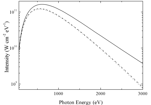
FIG. 22: Comparison of spectra incident on the center of the sample in our standard ( l = 1150 \mu\text{m} ) halfraum at t = 1.0 ns, with the standard beam pointing. The dotted line represents the simulation with no foil, the dashed line (nearly coincident with the dotted line) represents the simulation with a foil outside the LEH, and the solid line is from the simulation with the foil heated by ten beams.
