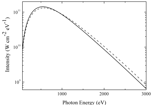
FIG. 9: Comparison of the spectrum incident on a sample at the center of a hohlraum when it is oriented toward the LEH (dotted line, 0 degree case in the previous figure) vs. the spectrum when the sample is oriented toward the hohlraum wall (solid line, 90 degree case in the previous figure). The LEH-facing sample has a significantly harder spectrum, though the radiation temperature onto each is nearly identical (190 eV vs. 191 eV).
