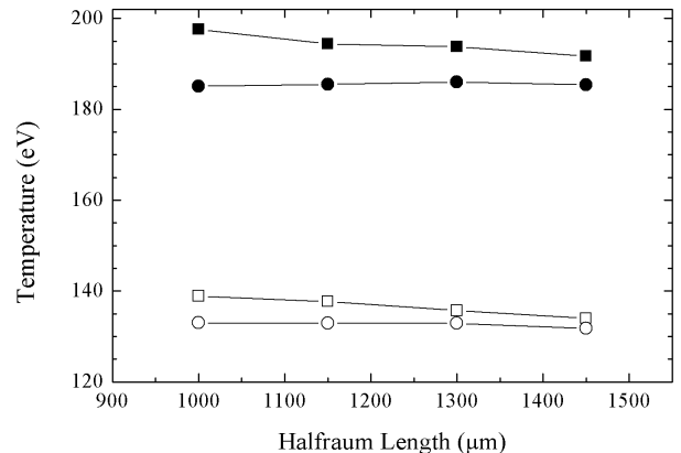
FIG. 20: Temperature as a function of halfraum length, where the beam pointing is changed along with halfraum length, such that the hot spots' distance from the sample mounted on the back wall is always the same (mean hot spot distance of 530 \mu\text{m} from the back wall, measured along the barrel). The solid symbols are from a simulation time of t = 1.0 \text{ ns} while the open symbols are from t = 100 \text{ ps} . The squares are DANTE temperatures and the circles are sample radiation temperatures.
