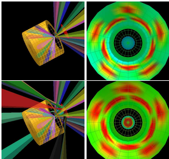
FIG. 21: Two halfraum simulations with a metal foil just outside the LEH. In the simulation shown in the top two panels, there are no beams onto the foil. The foil simply acts to absorb and reemit radiation that exits through the LEH. In the bottom two panels, there are ten beams onto the foil, which significantly increases the radiation flux inside the halfraum. All the snapshots show emission temperatures at t = 1.0 ns.
