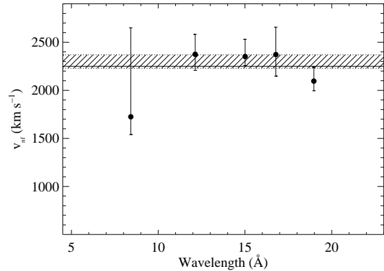
Figure 11. Values of the terminal velocity derived from fitting five strong lines with a wind profile model for which v_\infty was allowed to be a free parameter (along with \tau_* , R_0 , and the normalization). The bulk wind terminal velocity adopted from the analysis of UV profiles is indicated by the solid horizontal line. The cross-hatched area represents the 68 percent confidence region for the value of the terminal velocity derived from fitting these five points.
