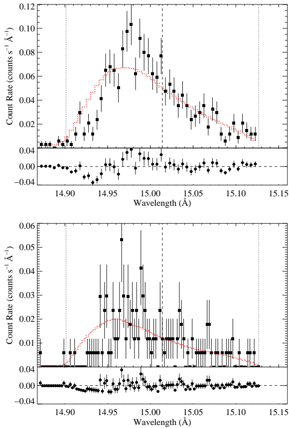
Figure 5. The Fe XVII line at 15.014 Å in the MEG (top) and HEG (bottom), with the best-fit model having \tau_* = 4.58 superimposed. This model fit is statistically unacceptable.
