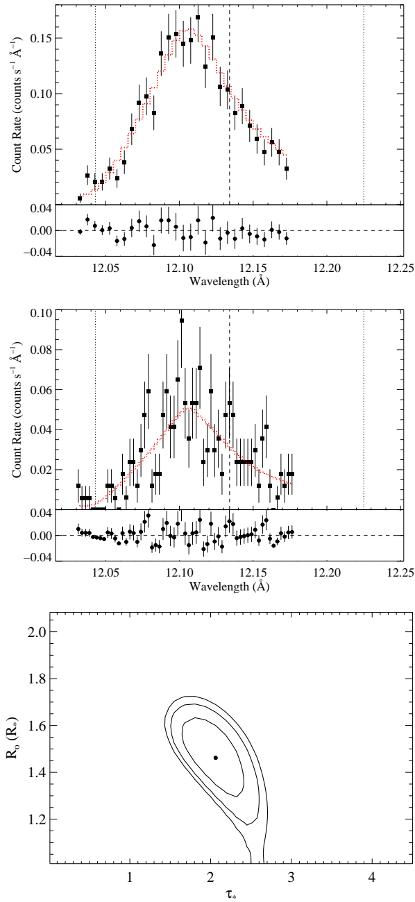
Figure 8. The MEG (top) and HEG (middle) measurements of the Ne X Ly \alpha line at 12.134 Å, along with the best-fit model. This line shows an intermediate degree of blue shift and asymmetry, indicative of an intermediate \tau_* value, as is expected at its wavelength, where the wind opacity is larger than at the wavelength of the Mg XII Ly \alpha line, but not as large as at longer wavelengths. We also show the 68, 90, and 95 percent confidence limits in \tau_* , R_o parameter space (bottom).
