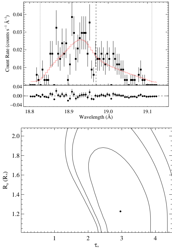
Figure 9. The MEG (top) measurements of the O VIII Ly \alpha line at 18.969 Å, along with the best-fit model. This line shows a relatively large degree of blue shift and asymmetry, indicative of a higher \tau_* value, as is expected at longer wavelengths, where the wind opacity is larger. We did not include the very weak HEG data in the analysis of this line. We also show the 68, 90, and 95 percent confidence limits in \tau_* , R_o parameter space (bottom).
