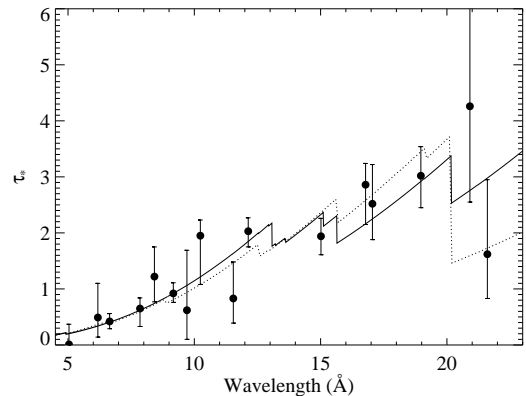
Figure 14. The best-fit model, with \dot{M} = 3.88 \times 10^{-6} , shown in Fig. 13, is shown here again, but this time it is compared to the best-fit solar abundance \tau_* model (dotted curve). The fits are of similar quality, while the solar abundance model has a lower mass-loss rate ( \dot{M} = 1.90 \times 10^{-6} ) to compensate for its higher overall opacity.
