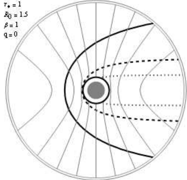
Figure 2. A visualization of the wind Doppler shift and optical depth – two effects that govern the observed, broadened and asymmetric line shapes. The observer is on the left, and the light solid contours represent the line-of-sight velocity in increments of 0.2v_{\infty} , with the blue shifts arising in the left hemisphere and the red shifts in the right. The star is the gray circle at the center, and the inner radius of the wind X-ray emission, R_o , is indicated at 1.5 R_* by the solid black circle. The solid heavy contour represents the locus of points with optical depth \tau = 0.5 , and the dashed and dotted contours represent \tau = 1 and 2 , respectively. The model parameters visualized here are nearly identical to those of the best-fitting model for the Mg XII Ly \alpha line shown in Fig. 7. Note to coauthors: We will clean this figure up, removing the parameter labels in the upper left, incorporating them into the caption, and perhaps labeling some of the contours.
