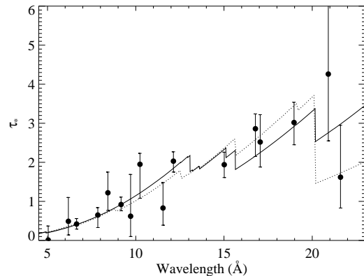
Figure 14. The best-fit model, with \dot{M} = 3.88 \times 10^{-6} , shown in Fig. 13, is shown here again, but this time it is compared to the best-fit solar abundance \tau_* model (dotted curve). The fits are of similar quality, while the solar abundance model has a lower mass-loss rate ( \dot{M} = 1.90 \times 10^{-6} ) to compensate for its higher overall opacity.
