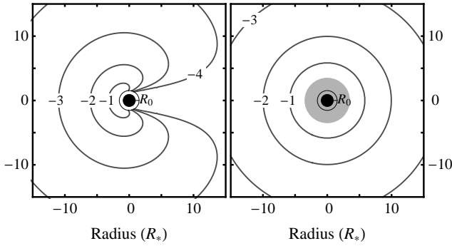
Figure 2. The left panel is the same as Figure 1, but plotting the renormalized product of emissivity times transmission, including occultation by the stellar core. The right panel shows the same plot in the exospheric approximation, where the grey zone is inside the radius of (radial) optical depth unity and thus does not contribute to the observed X-ray flux.
