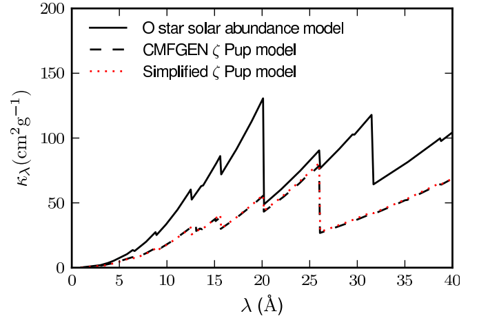
Figure 7. Comparison of three different model O star wind opacities: the solar abundance O star wind model shown in Fig 6 (solid); an CMFGEN model appropriate for \zeta Pup (dashed) using the abundances of Bouret et al. (in preparation); and a simplified version of this CMFGEN model (dotted; red in the electronic version) where the ionization balance is the same as in the solar abundance model. Note that the Bouret et al. abundances for \zeta Pup are sub-solar as well as having altered CNO abundance ratios.
