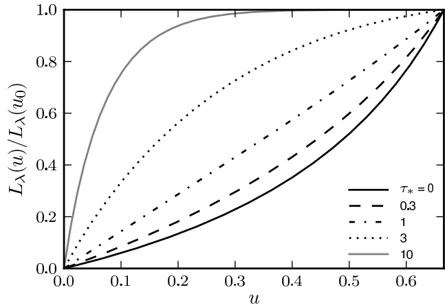
Figure 4. Fraction of X-ray emission originating from outside inverse radius u , normalized to total X-ray emission integrated to u_0 . For all but the very optically thick case of \tau_* = 10 , the emission comes from a wide range in u .
