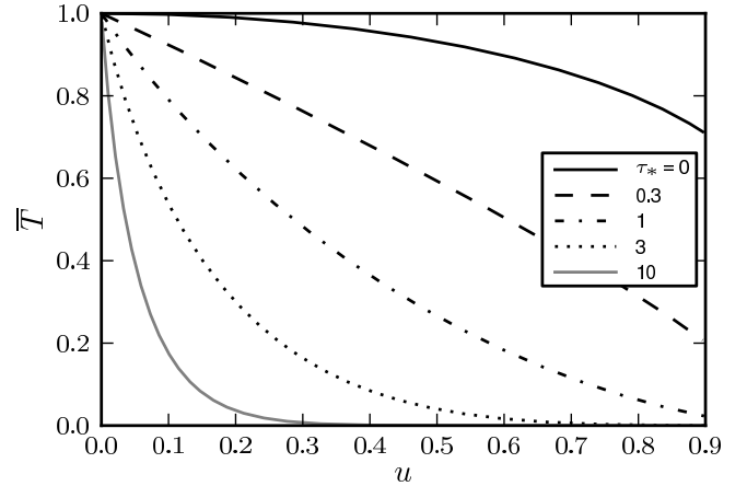
Figure 3. Angle averaged transmission \bar{T} as a function of shell inverse radial coordinate u = R_*/r , with different curves for different characteristic wind optical depths \tau_* . The equivalent plot in the exospheric approximation would be a step function at u_1 , the inverse radial coordinate of optical depth unity. Note that the transmission is less than unity even for \tau_* = 0 due to occultation by the stellar core.
