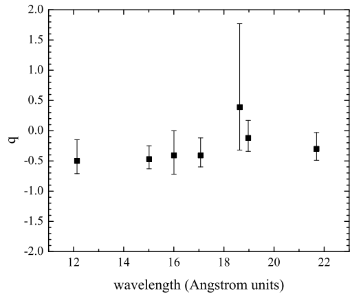
Figure 6. The best-fit model parameters – \tau_* , q , and R_{\min} – for each line complex we fit with a wind-profile model. The error bars represent the 90% confidence limits on the one parameter of interest in each panel ( \Delta C = 2.71 ).
