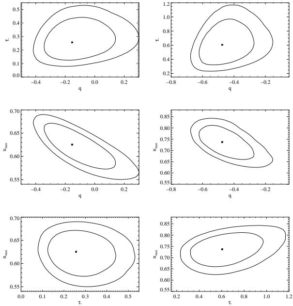
Figure 5. The 68% and 90% confidence regions in the parameter space of the wind-profile model, for the two lines shown in Figure 2, the O VIII Ly _{\alpha} line (left-hand column) and the Fe XVII 15.014 Å line (right-hand column). The best-fit model parameters are indicated by the asterisks. Note the correlation between q and R_{\min} ( u_{\max}^{-1} ). For each 2-D slice of parameter space shown here, the other model parameters are optimized (i.e. free) while models are fit for a grid of the two displayed parameter values. The contour levels thus correspond to \Delta C values appropriate for two parameters of interest: 2.30 and 4.61.
