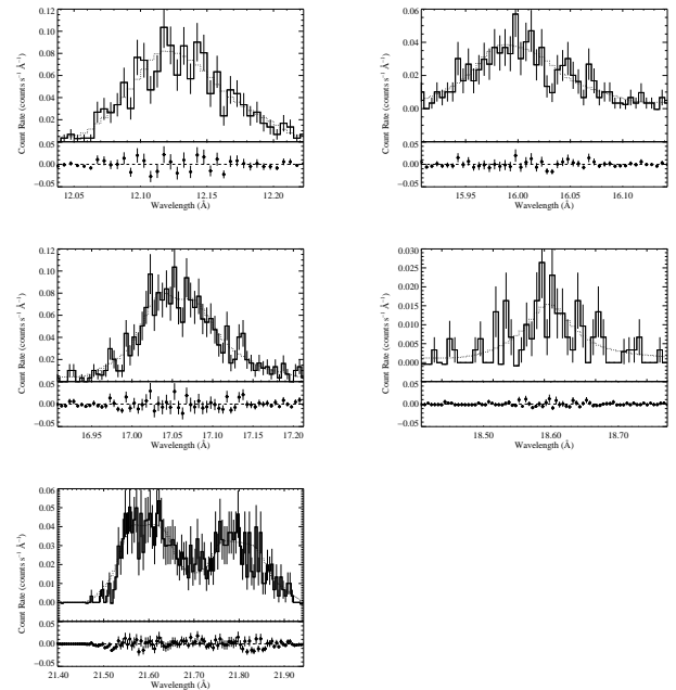
Figure 4. Best-fit wind-profile models for five lines (or line complexes): Ne X 12.134 Å, O VIII 16.006 Å, Fe XVII 17.051 Å and 17.096 Å, O VII 18.627 Å, and O VII 21.602 Å and 21.804 Å.
