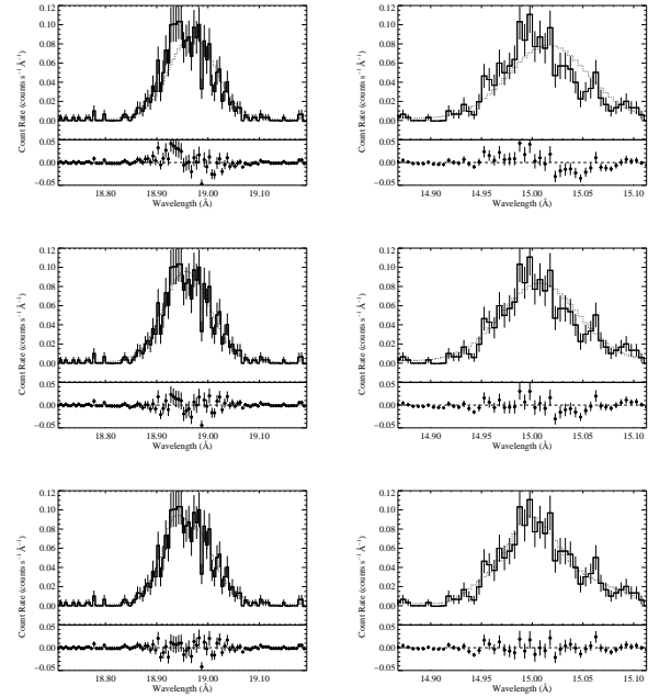
Figure 2. Best-fit models superimposed on the observed O VIII Ly \alpha line (left-hand column) and the Fe XVII 15.014 \text{\AA} line (right-hand column). Error bars here and in other figures are calculated from the total source counts per bin, assuming Poisson errors. The fits shown in the top row are for a Gaussian model with the line center fixed at the laboratory rest wavelength. This fits shown in the middle row are for the Gaussian model with the centroid treated as a free parameter. The Gaussian fits in the first two rows are discussed in Sec. 3. The fits shown in the lower panel are for the wind-profile model discussed in Sec. 4.
