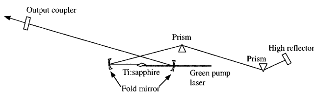
FIG. 2. Schematic diagram of a self-modelocked Ti:sapphire laser.
