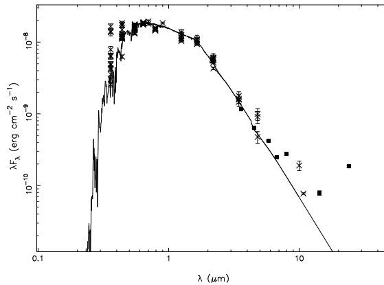
Fig. 1.— Example figure: The spectral energy distribution of DoAr 21, from ultraviolet ( 4000 \text{ \AA} ) through infrared wavelengths. Spitzer and ISO data are shown as filled squares, and the 850 \mu\text{m} and 1.3 \text{ mm} upper limits are not shown. The photometry has been de-reddened with A_V = 6.2 and R_V = 4.2 as described in the text. Overplotted is a model photosphere (solid line); the star shows a clear infrared excess at \lambda \geq 8 \mu\text{m} .
