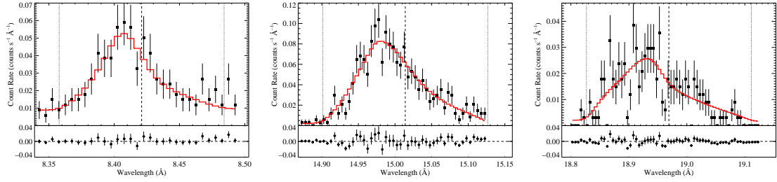
FIGURE 2. In these three panels are three separate emission lines from the Chandra spectrum of the massive star \zeta Puppis. These are, from left to right, the Ly \alpha line of Mg XII at 8.42 \text{\AA} , the Fe XVII line at 15.01 \text{\AA} which is the 3C transition from the 3d^1P_1 level to the ground state, and the Ly \alpha line of O VIII at 18.97 \text{\AA} . The laboratory rest wavelengths for each emission line are indicated by the vertical dashed lines while the Doppler shifts associated with the stellar wind terminal velocity are represented by the light dashed vertical lines. The data are the points with (Poisson) error bars, the model is shown as the solid (red) histogram, and the fit residuals are shown in the horizontal windows below each data plot. The values of R_0 , the onset radius of x-ray emission we find for each line, are R_0 = 1.34^{+0.22}_{-0.18} , 1.55^{+0.13}_{-0.12} , and 1.18^{+0.41}_{-0.17} R_* for the Mg, Fe, and O lines, respectively. This is consistent with the predictions of the LDI wind-shock model, in which strong shocks start to form several tenths of a stellar radius above the photosphere. The values we derive for the \tau_* parameter from the profile model fitting are \tau = 1.22^{+0.53}_{-0.45} , 1.94^{+0.32}_{-0.33} , and 3.02^{+0.52}_{-0.57} . Note that these values are consistent with the wavelength dependence of the atomic opacity of the wind, as expected.
