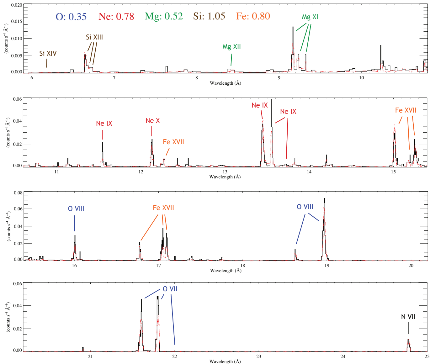
Figure 5. The best-fit two-temperature, variable abundance thermal spectral (APEC) model (dotted line; red in on-line color version; parameters listed in Tab. 3), superimposed on the adaptively smoothed co-added MEG first-order spectrum. Emission lines are labeled and color coded according to element, with the abundances of each element listed at the top of the figure. Some non-detected lines are labeled, including the forbidden line of O VII near 22.1 Å and the Lyman-alpha line of Si XIV near 6.2 Å. The nitrogen Lyman-alpha line is labeled in black, as we cannot accurately constrain its abundance because only one line is measured.
