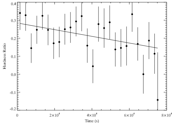
Figure 17. The hardness ratio as a function of time, defined as HR \equiv \frac{CR(>1\text{keV}) - CR(<1\text{keV})}{CR(>1\text{keV}) + CR(<1\text{keV})} , where the CR denotes the count rate in the combined zeroth order and first order (MEG) data, over the indicated photon energy ranges. We fit a linear function to the data, and find \chi^2 = 25 for 24 degrees of freedom for a constant model (slope of zero), so a constant source model cannot be rejected outright. However, the best-fit slope of -1.9 \times 10^{-6} cts \text{s}^{-2} gives \chi^2 = 20 , which is a statistically significant improvement.
