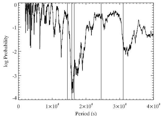
Figure 11. Rejection probability (significance level increasing downward) of assumed period, according to the Kuiper statistic. The five known optical pulsation periods (Aerts et al. 1998; Cuypers et al. 2002) are indicated by the vertical lines. The primary pulsation period is the third of these.
