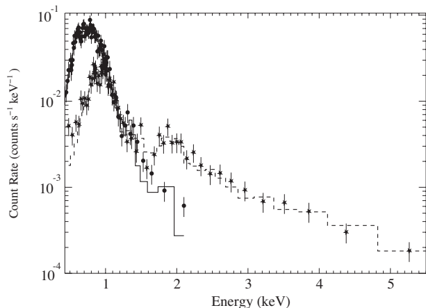
Figure 13. The zeroth order spectrum of the companion (stars) is shown along with that of \beta Cru (circles). The companion's spectrum is significantly harder, and is well-fit by a two-temperature thermal model with component temperatures several times higher than those found for \beta Cru.
