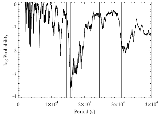
Figure 10. Rejection probability (significance level increasing downward) of assumed period, according to the Kuiper statistic. The five known optical pulsation periods (Aerts et al. 1998; Cuyppers et al. 2002) are indicated by the vertical lines. The primary pulsation period is the third of these.
