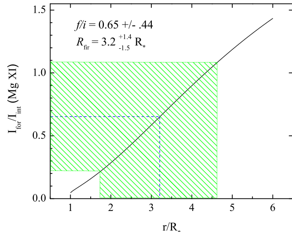
Figure 9. The Mg XI resonance-intercombination-forbidden complex in the co-added MEG data, with the best-fit wind-profile models overplotted (top). The constraints on the formation radius, R_{\text{fir}} , are shown in the bottom panel.
