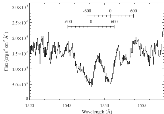
Figure 6. The C IV resonance doublet from several coadded archived IUE observations. A velocity scale ( \text{km s}^{-1} ) in the frame of the star is shown above the data. These lines show the characteristic blue-shifted absorption that is expected from a stellar wind, but the lines are not only weak compared to theoretical expectations but also much less wind broadened.
