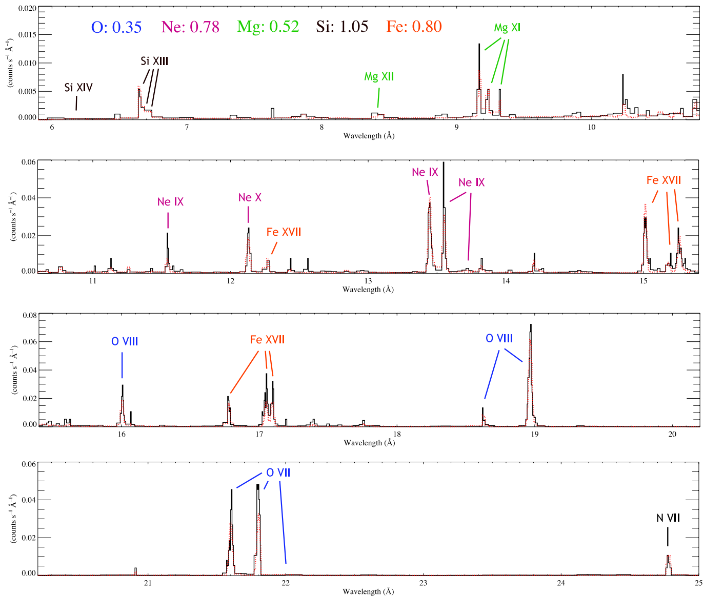
Figure 4. The best-fit two-temperature, variable abundance thermal spectral (APEC) model (dotted line; red in on-line color version; parameters listed in Tab. 3; same model as shown in Fig. 3), superimposed on the adaptively smoothed co-added MEG first-order spectrum of \beta Cru. Emission lines are labeled and color coded according to element, with the abundances of each element listed at the top of the figure. Some non-detected lines are labeled, including the forbidden line of O VII near 22.1 Å and the Lyman-alpha line of Si XIV near 6.2 Å. The N Lyman-alpha line is labeled in black, as we cannot accurately constrain its abundance because only one line is measured.
