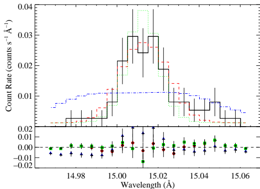
Figure 7. The Fe XVII line at 15.014 Å with three different wind profile models. The dashed line (red in on-line color version) is a constant-velocity wind model with v_\infty = 280 \text{ km s}^{-1} (the best-fit value for a constant outflow velocity, which produces emission lines with v_{\text{hwhm}} \approx 150 \text{ km s}^{-1} ). The model with v_\infty = 2000 \text{ km s}^{-1} , \beta = 1 , and R_{\text{min}} = 1.5 R_\star is represented by the dot-dash line (blue in on-line color version). An infinitely narrow model is shown as the dotted line (green in on-line color version). The residuals for each model fit are shown in the lower panel, as red circles for the global best-fit, modestly broadened ( v_\infty = 280 \text{ km s}^{-1} ) model, green squares for the narrow profile model, and blue triangles for the broad wind model. The wind model with the higher velocity ( v_\infty = 2000 \text{ km s}^{-1} ) clearly does not provide a good fit, while the narrower constant velocity ( v_\infty = 280 \text{ km s}^{-1} ) wind model does. And while the very narrow model cannot be absolutely ruled out, the v_\infty = 280 \text{ km s}^{-1} model is preferred over it with a high degree of significance. All the models shown here have been convolved with the instrumental response function.
