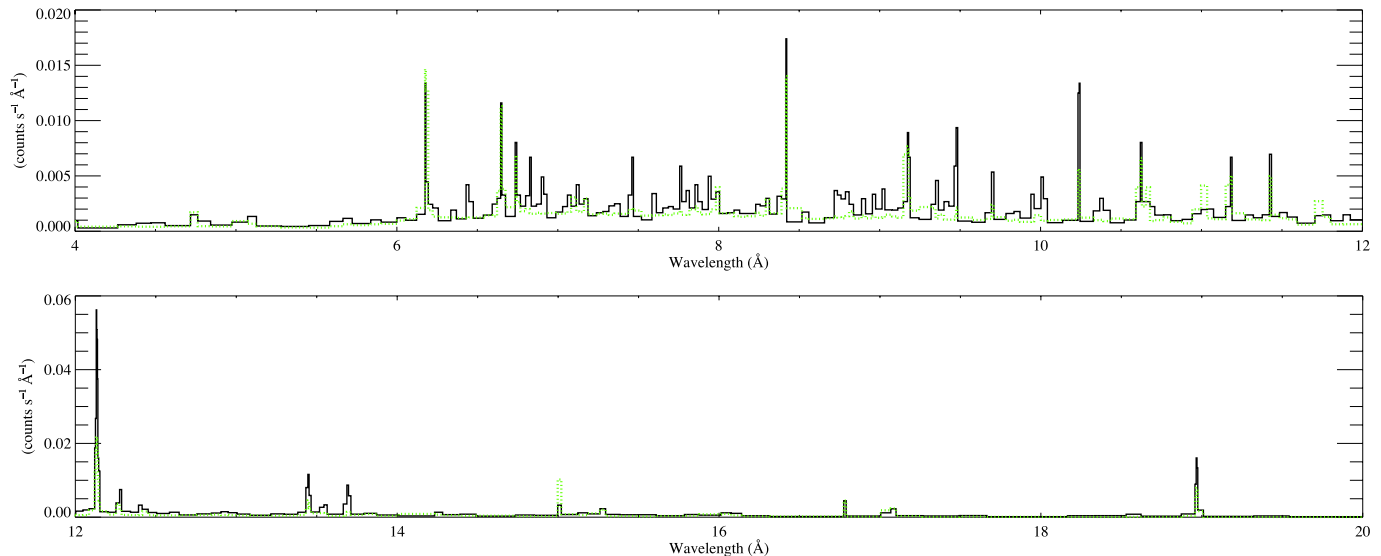
Figure 13. The best-fit two-temperature, variable abundance thermal spectral (APEC) model (dotted line; green in on-line color version), superimposed on the adaptively smoothed co-added MEG first-order spectrum of the companion (solid, black line).
