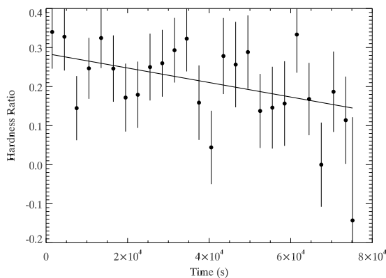
Figure 15. The hardness ratio as a function of time, defined as HR \equiv \frac{CR(>1\text{keV}) - CR(<1\text{keV})}{CR(>1\text{keV}) + CR(<1\text{keV})} , where the CR denotes the count rate in the combined zeroth order and first order (MEG) data, over the indicated photon energy ranges. We fit a linear function to the data, and find \chi^2 = 25 for 24 degrees of freedom for a constant model (slope of zero), so a constant source model cannot be rejected outright. However, the best-fit slope of -1.9 \times 10^{-6} cts \text{s}^{-2} gives \chi^2 = 20 , for 23 degrees of freedom, which is a statistically significant improvement.
