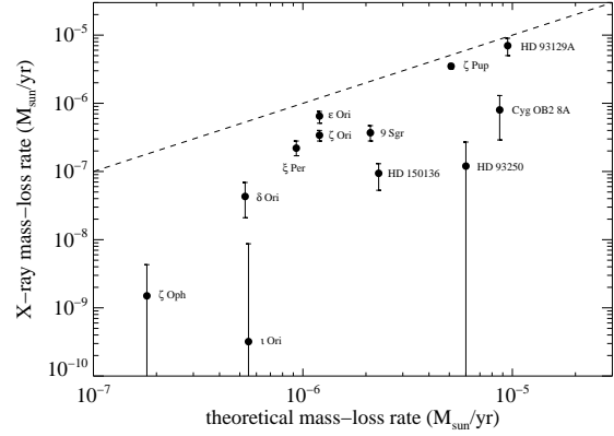
Figure 6. The X-ray derived mass-loss rates for each star in our sample (and also \zeta Pup and HD 93129A) compared to the theoretically expected mass-loss rate from Vink et al. (2000). The dashed line is the locus where these two quantities are equal.
