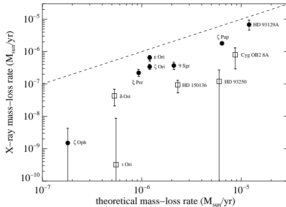
Figure 6. The X-ray derived mass-loss rates for each star in our sample (and also \zeta Pup and HD 93129A) compared to the theoretically expected mass-loss rate from Vink et al. (2000). Stars dominated by EWS are shown as filled circles, while those where our model breaks down, in most cases due to CWB X-rays, are shown as open squares.
