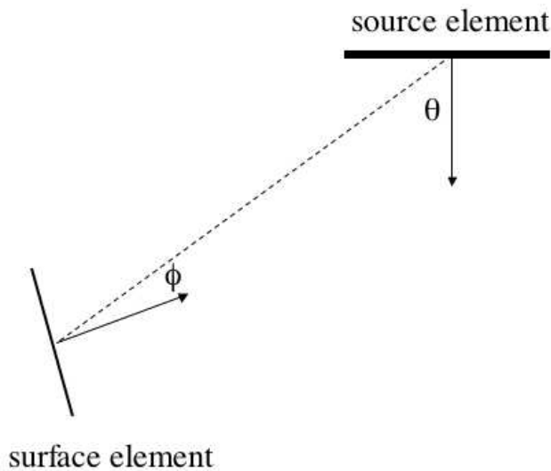
FIG. 2: Schematic of the view-factor calculation for an arbitrary geometry. The flux from any source surface element onto any other sample surface element is proportional to the cosine of the angle between the line of centers of the two elements and the surface normal of the source element (because the source element is assumed to be a Lambertian emitter) and also to the cosine of the line of centers and the normal of the sample element (accounting for the projected cross section of the sample as seen by the source). The line of centers are indicated by the dashed line while the two surface normals are indicated by arrows.
