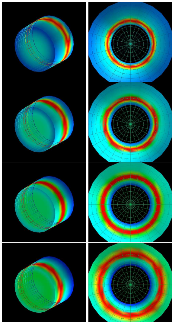
FIG. 11: Series of four halfraum simulations in which the beam pointing was varied. These are identical to the series shown in Fig. 9, except that the LEH is larger in these targets, with a diameter equal to the diameter of the halfraum itself ( i.e. no lip on the LEH). The pairs of images show the DANTE view on the left and the view from behind the sample on the far wall, or end cap, of the halfraum on the right, both at t = 1.0 ns. The top row has the beams pointed closest to the LEH, with the pointing moving in by 150 \mu\text{m} at each simulation, moving down the figure.
