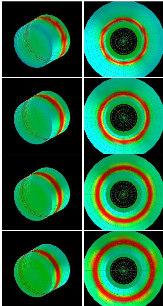
FIG. 9: Series of four halfraum simulations in which the beam pointing was varied. The pairs of images show the DANTE view on the left and the view from behind the sample on the far wall, or end cap, of the halfraum on the right, both at t = 1.0 ns. The top row has the beams pointed closest to the LEH, with the pointing moving in by 150 \mu\text{m} at each simulation, moving down the figure. This series of simulations has the beams pointed so that the hot spots make a single ring, and the halfraum has a three-quarter LEH.
