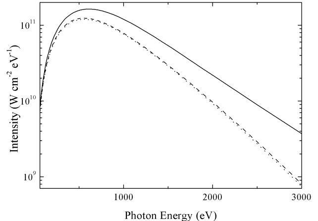
FIG. 20: Comparison of spectra incident on the center of the sample in our standard ( l = 1150 \mu\text{m} ) halfraum at t = 1.0 ns, with the standard beam pointing. The dotted line represents the simulation with no foil, the dashed line (nearly coincident with the dotted line) represents the simulation with a foil outside the LEH, and the solid line is from the simulation with the foil heated by ten beams.
