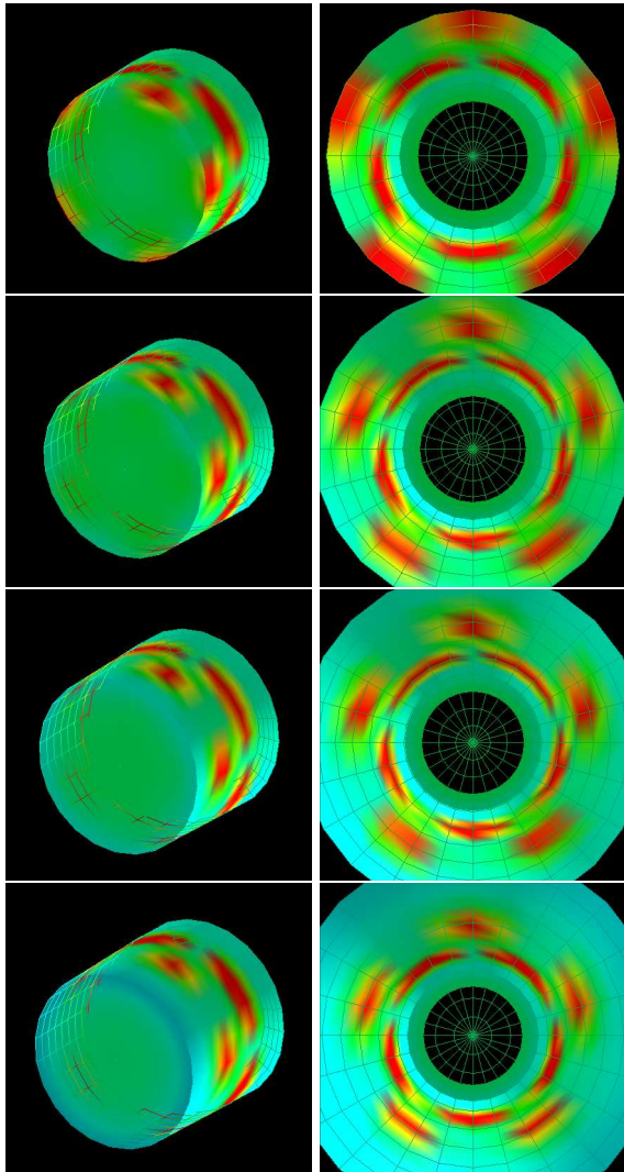
FIG. 15: Series of four halfraum simulations in which the length of the halfraum was varied. From top to bottom, the halfraum lengths are 1000, 1150, 1300, and 1450 \mu\text{m} . The beam pointing and focus was at the LEH center in all cases. The left hand column shows the DANTE view and the right hand column the sample view. The colors represent emission temperatures taken from t = 1.0 ns in each simulation.
