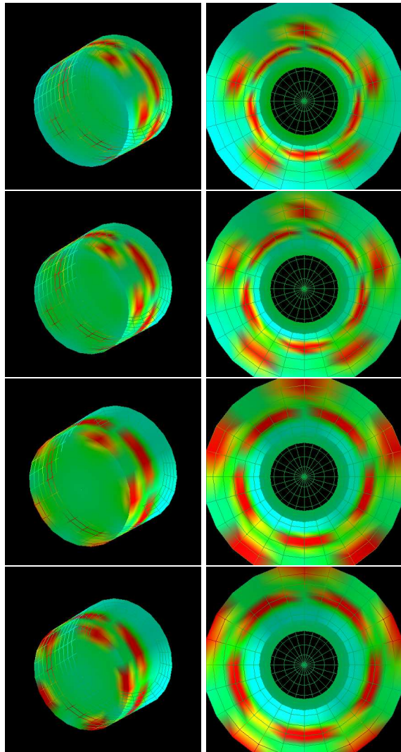
FIG. 13: Final series of four halfraum simulations, in which the beam pointing was varied. The beam pointing here gives two separate rings for Cones 2 and 3, respectively, and we revert to the standard three-quarter LEH. The beams are moved inward by 150 \mu\text{m} each step down the figure, with the second row representing the nominal pointing (all beams pointed at the center of the LEH). The left hand column shows the DANTE view, the right hand column shows the sample view. The colors represent emission temperatures at t = 1.0 \text{ ns} .
