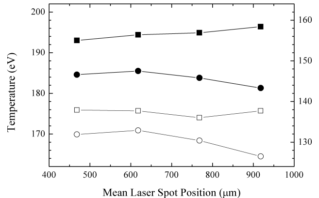
FIG. 14: Temperature as a function of pointing for the third set of simulations described in this section, with the two beam cones making two different rings of hot spots, and using the three-quarter LEH. The solid symbols are from a simulation time of t = 1.0 ns (left-hand axis) while the open symbols are from t = 100 ps (right-hand axis). The squares are DANTE temperatures and the circles are sample radiation temperatures. The spot position is measured along the barrel, from the LEH plane.
