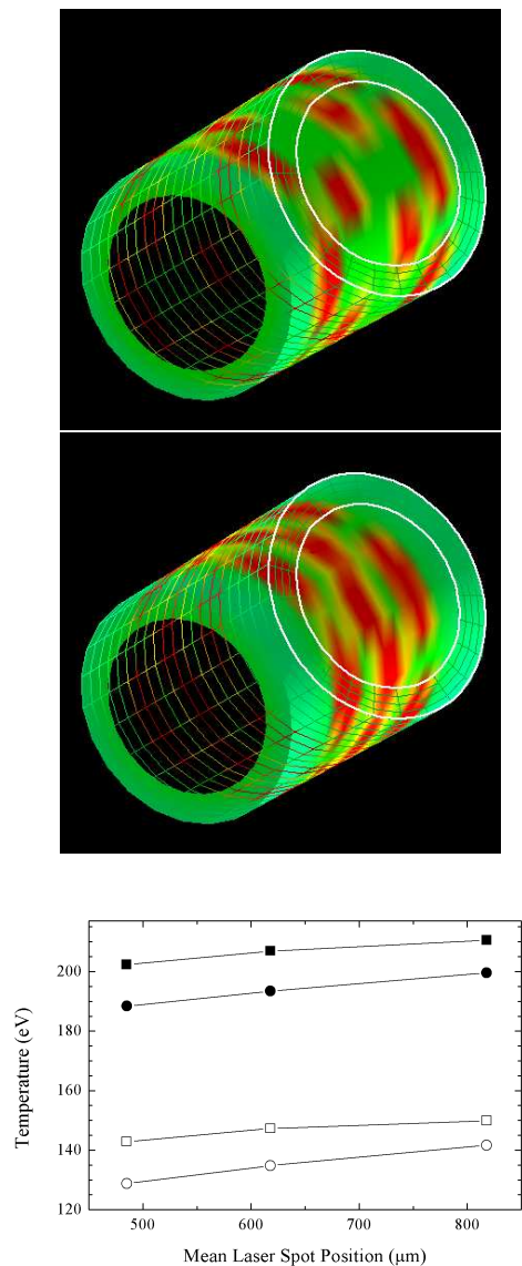
FIG. 5: The DANTE views of the hohlraum in the two cases with different beam pointings (top two panels). As in the bottom panel of Fig. 1, we show a color map of emission temperature at t = 1.0 ns, and hide the beams for clarity. The color scale spans 140 eV to 220 eV, and as is true for all the color figures throughout the paper, it is identical to the map shown at the bottom of Fig. 1. The lower panel shows the trends of DANTE temperature (squares) and midplane temperature (circles) as the beam pointing is changed. The filled symbols represent simulation time t = 1.0 ns (XCE = 0.55 and albedo = 0.73) and the open symbols represent simulation time t = 100 ps (XCE = 0.28 and albedo = 0.18). The original model, used to reproduce the experiments reported on in [4], has a mean laser spot position 480 \mu\text{m} from the LEH plane. The first variation ( 620 \mu\text{m} ) is shown in the top panel and the second variation ( 820 \mu\text{m} ) is shown in the middle panel. We note that in this last case, the Cone 2 beams from either side of the hohlraum hit the wall almost exactly at the midplane, creating a single, combined ring of hot spots.
