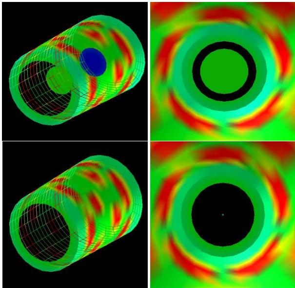
FIG. 17: Emission temperature color maps at, t = 1 ns, of the hohlraum simulation with the LEH shields (top row) compared to an identical simulation without shields (bottom row; same simulation as that shown in the top panel of Fig. 5). The left column shows the usual DANTE view, while the right column shows a view from near the hohlraum midplane, looking toward one of the LEHs.
