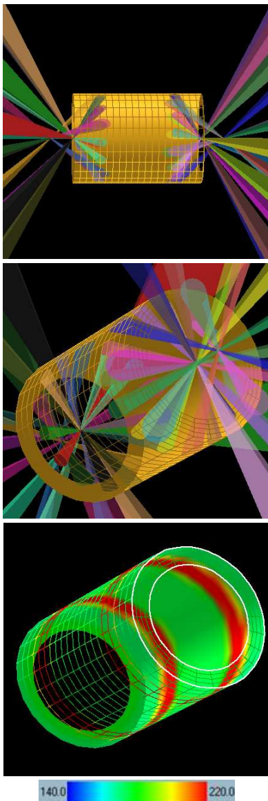
FIG. 1: Hohlräum images generated with the VISRAD view-factor code, relevant to the experiments discussed in reference [4]. The top panel shows the OMEGA beam pointing into the hohlraum cylinder seen side-on. Note that the Cone 2 beams on each side are pulled back so that the beams from both cones make a single ring on each side of the hohlraum. The middle panel shows the same target model, but from the position of the DANTE diagnostic. The lower panel shows the DANTE view again, but with the beams hidden, and with the wall temperature at t = 1.0 ns displayed as a color map (the dynamic range in this, and all other, temperature color maps shown in the paper is 140 eV to 220 eV). Note the ring of laser hot spots on each side of the hohlraum. Note also in all of these images how structures in the model seen from the back, or outside, are rendered as transparent mesh to allow for an unobstructed view of the interior of the hohlraum. This convention will be used throughout the paper. Finally, we point out that the “front,” DANTE-facing, LEH is in the upper right in this, and all similar figures throughout the paper, and the inner and outer edges of the front LEH lip are highlighted in white.
