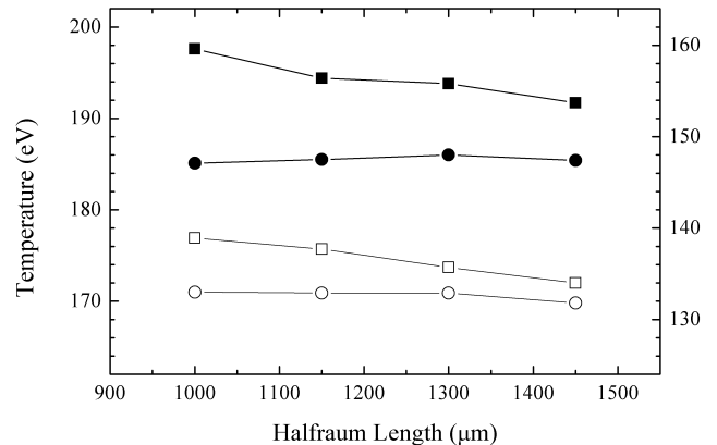
FIG. 16: Temperature as a function of halfraum length, where the beam pointing is changed along with halfraum length, such that the hot spots’ distance from the sample mounted on the back wall is always the same (mean hot spot distance of 530 \mu\text{m} from the back wall, measured along the barrel). The solid symbols are from a simulation time of t = 1.0 ns (left-hand axis) while the open symbols are from t = 100 ps (right-hand axis). The squares are DANTE temperatures and the circles are sample radiation temperatures.
