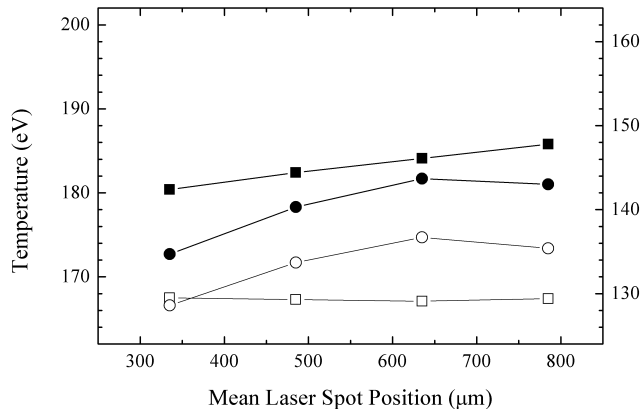
FIG. 13: The radiation temperature on a sample mounted on the end of a halfraum (circles) and measured by DANTE (squares) for the four different beam pointings at two different simulation times: t = 1.0 ns (filled symbols; left-hand axis) and t = 100 ps (open symbols; right-hand axis). In these simulations there is no LEH lip ( i.e. 100% LEH) and the beams are pointed to form a single ring of hot spots. The spot position is measured along the barrel, from the LEH plane.
