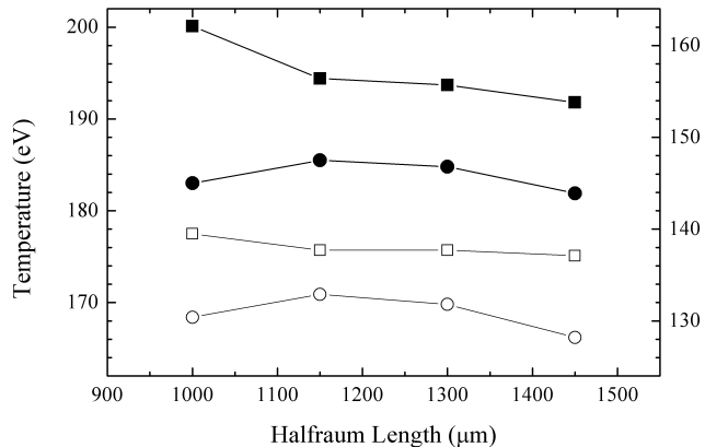
FIG. 15: Temperature as a function of halfraum length for four simulations having identical beam pointings with respect to the LEH. The solid symbols are from a simulation time of t = 1.0 ns (left-hand axis) while the open symbols are from t = 100 ps (right-hand axis). The squares are DANTE temperatures and the circles are sample radiation temperatures.
