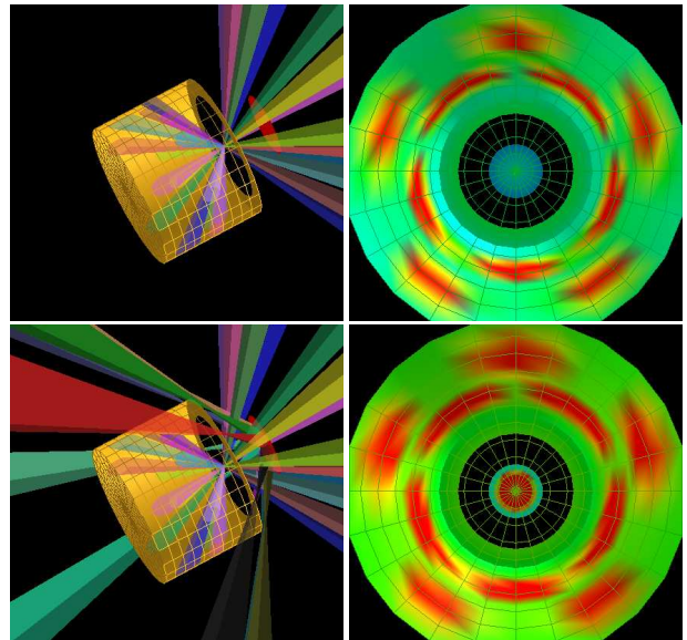
FIG. 18: Two halfraum simulations with a metal foil just outside the LEH. In the simulation shown in the top two panels, there are no beams onto the foil. The foil simply acts to absorb and reemit radiation that exits through the LEH. In the bottom two panels, there are ten beams onto the foil, which significantly increases the radiation flux inside the halfraum. All the snapshots show emission temperatures at t = 1.0 ns.
