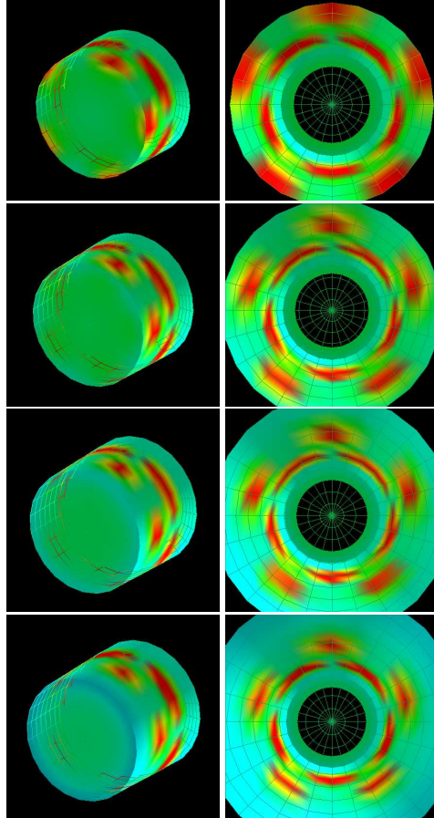
FIG. 17: Series of four halfraum simulations in which the length of the halfraum was varied. From top to bottom, the halfraum lengths are 1000 , 1150 , 1300 , and 1450 \mu\text{m} . The beam pointing and focus was at the LEH center in all cases. The left hand column shows the DANTE view and the right hand column the sample view. The colors represent emission temperatures taken from t = 1.0 ns in each simulation.
