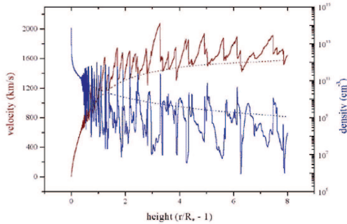
Figure 5. A snapshot showing the velocity (increasing with height; left-hand axis) and density (decreasing with height; right-hand axis) as a function of height above the photosphere in a radiation hydrodynamics simulation of the wind of \zeta Pup. Shock-heated plasma cools rapidly; the bulk of the wind in any given snapshot is cold.
