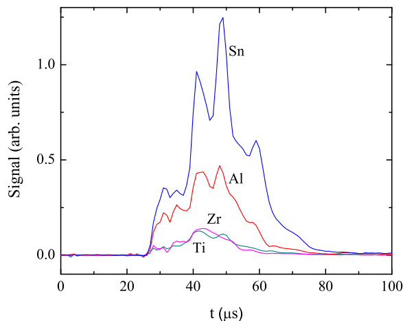
FIG. 11: (Color) SXR data from a discharge with counter-helicity merging, smoothed over 1 \mu\text{s} intervals. Note the onset of strong soft X-ray emission around 30\text{-}40 \mu\text{s} , when reconnection begins.
