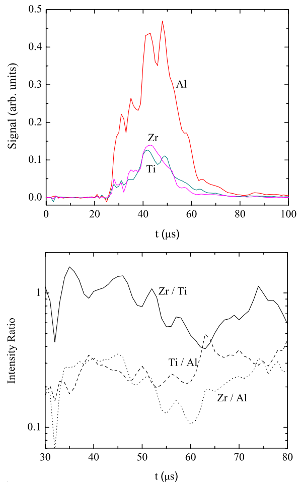
FIG. 12: (Color) Top: SXR data for the Al, Zr, and Ti filters from a discharge with counter-helicity merging, smoothed over 1 \mu\text{s} intervals. Bottom: Time evolution of filter ratios for the discharge. Sn filter data is omitted in order to more clearly show the time evolution of the other three ratios.
