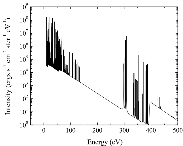
FIG. 13: Model spectrum from a steady-state simulation with T_e = 30 eV and n_i = 5 \times 10^{14} \text{ cm}^{-3} . Impurity concentrations of 1% carbon, 0.002% oxygen, and 0.003% nitrogen were included. The plasma emits primarily at E < 150 eV, but SXR will also measure substantial emission from the C v and C VI resonance lines between 300 and 400 eV. Note that the Zr channel has the lowest responsivity at these energies, which is counter to what is seen below 100 eV.
