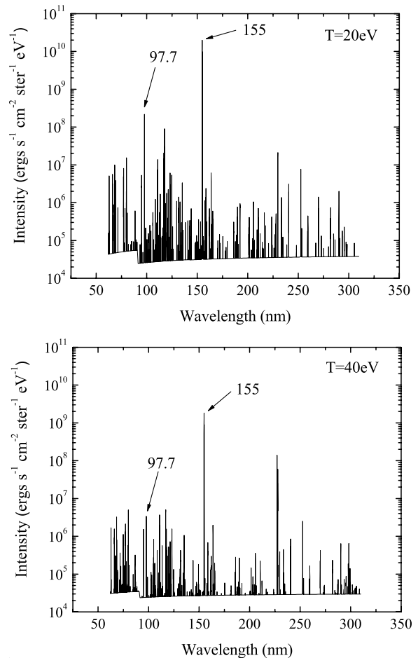
FIG. 2: Model spectra from steady-state simulations with T_e = 20 \text{ eV} (top) and T_e = 40 \text{ eV} (bottom). Both simulations assume a uniform 40 cm thick plasma composed of 99% hydrogen and 1% carbon with an ion density of 5 \times 10^{14} \text{ cm}^{-3} . The temperature dependence of the I_{97.7}/I_{155} line ratio is evident. Note also the presence of the Lyman edge at 91.2 nm, indicating that radiative recombination of hydrogen, rather than bremsstrahlung, is the dominant continuum process at work.
