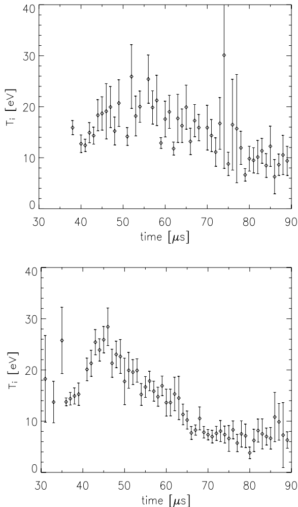
FIG. 8: Thermal Doppler broadening of the C III 229.687 nm line observed with the IDS instrument viewing along a mid-plane diameter of the plasma during counter helicity merging (top) and single spheromak discharges (bottom). Each data point is the average of up to ten discharges; data with small signal strength or showing nonthermal (flow profile) effects were dropped from the average.
