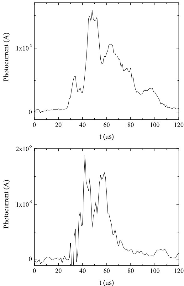
FIG. 5: Sample VUV monochromator data. Top: A measurement of the C IV 155 nm line intensity during a discharge with counter-helicity spheromak merging in SSX. Bottom: A measurement of the C III 97.7 nm line intensity during a single spheromak discharge.
