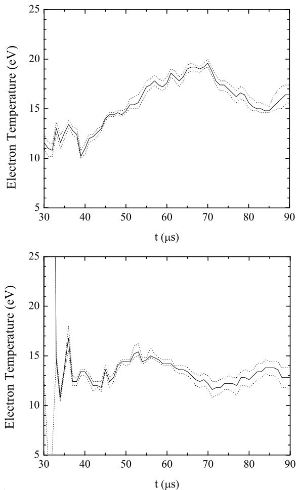
FIG. 7: Electron temperatures for counter helicity merging (top) and single spheromak discharges (bottom) derived from I_{97.7}/I_{155} measurements averaged over 25 discharges for each line. An ion density of 5 \times 10^{14} \text{ cm}^{-3} was assumed. Dashed lines give the uncertainty range, defined as the temperatures implied by a line ratio one standard deviation above or below the mean.
