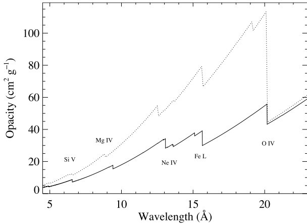
Figure 12. The wavelength dependent opacity of the wind of \zeta Pup computed using CMFGEN modelling of the ionization balance and sub-solar abundances derived from UV and optical spectra (solid), along with a solar-abundance opacity model (dotted). Note the prominent K-shell edge of oxygen near 20 Å in the solar abundance model. In the sub-solar metallicity opacity model, this decrement is much more modest, due to the underabundance of O and overabundance of N. The overall reduction in the opacity at most wavelengths in the CMFGEN model is the result of its overall subsolar metallicity and not its altered CNO abundances.
