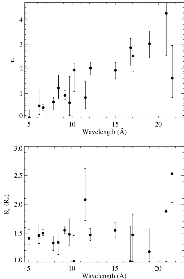
Figure 10. Values of \tau_* (top) and R_o (bottom) derived from the model fits, shown with their 68 percent confidence limits. Line complexes and blends that were fit with multiple model components are represented by only one point.
