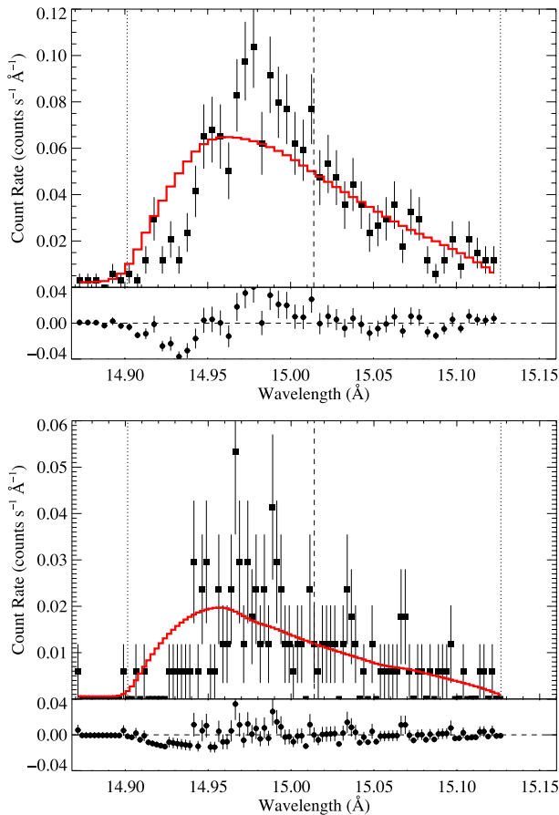
Figure 5. The Fe XVII line at 15.014 Å in the MEG (top) and HEG (bottom), with the best-fitting model having \tau_* = 5.30 superimposed. This is the value implied by the smooth-wind H \alpha mass-loss rate and our wind opacity model. The normalization and R_0 were the adjustable parameters of this fit. Even this best-fitting model is statistically unacceptable.
