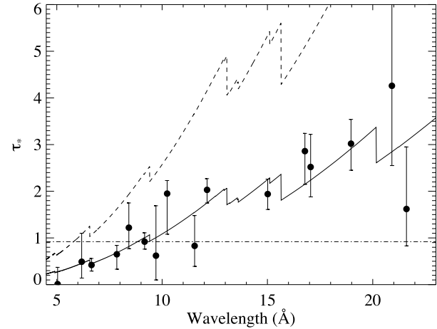
Figure 13. Values of \tau_* derived from the line-profile model fits, shown as points with error bars (same as the top panel of Fig. 10). The value of \tau_* expected if the mass-loss rate is 8.3 \times 10^{-6} M_{\odot} \text{ yr}^{-1} is shown as the upper dashed curve. Treating the mass-loss rate as a free parameter, the best fit value of 3.50 \times 10^{-6} M_{\odot} \text{ yr}^{-1} is shown as the lower, varying solid curve. This model provides a formally good fit. And both of these models of the wavelength-dependent \tau_* use the sub-solar metallicity (CMFGEN) opacity model. The horizontal dash-dot line is the best-fitting constant \tau_* model, as would be expected for a highly porous wind, where the effective opacity is completely determined by the macroscopic, physical cross sections of the optically thick clumps. It does not provide a good fit to the data.
