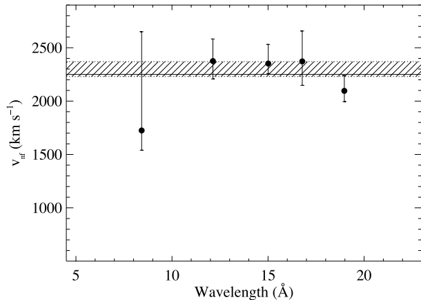
Figure 11. Values of the terminal velocity derived from fitting five strong lines with a wind profile model for which v_\infty was allowed to be a free parameter (the other parameters – \tau_* , R_* , and the normalization – were allowed to vary as well). The bulk wind terminal velocity adopted from the analysis of UV profiles is indicated by the solid horizontal line. The cross-hatched area represents the 68 percent confidence region for the value of the terminal velocity derived from fitting these five points.
