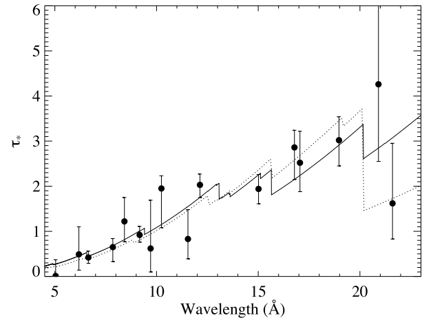
Figure 14. The best-fitting model, with \dot{M} = 3.50 \times 10^{-6} M_{\odot} \text{ yr}^{-1} , shown in Fig. 13, is shown here again, but this time it is compared to the best-fitting solar abundance \tau_* model (dotted curve). The fits are of similar quality, while the solar abundance model has a lower mass-loss rate ( \dot{M} = 1.90 \times 10^{-6} M_{\odot} \text{ yr}^{-1} ) to compensate for its higher overall opacity.
