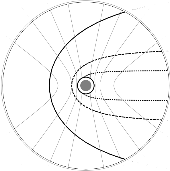
Figure 2. A visualization of the wind Doppler shift and optical depth – two effects that govern the observed, broadened and asymmetric line shapes. The observer is on the left, and the light contours represent the line-of-sight velocity in increments of 0.2v_\infty , with the blue shifts arising in the left hemisphere and the red shifts in the right. The star is the gray circle at the center, and the inner radius of the wind X-ray emission, R_o , is indicated at 1.5 R_* by the solid black circle. The solid heavy contour represents the locus of points with optical depth \tau = 0.33 , and the dashed and dotted contours represent \tau = 1 and 3 , respectively. The model parameters visualized here are nearly identical to those of the best-fitting model for the Ne x Ly \alpha line shown in Fig. 8 – R_o = 1.5 ; \tau_* = 2 .
